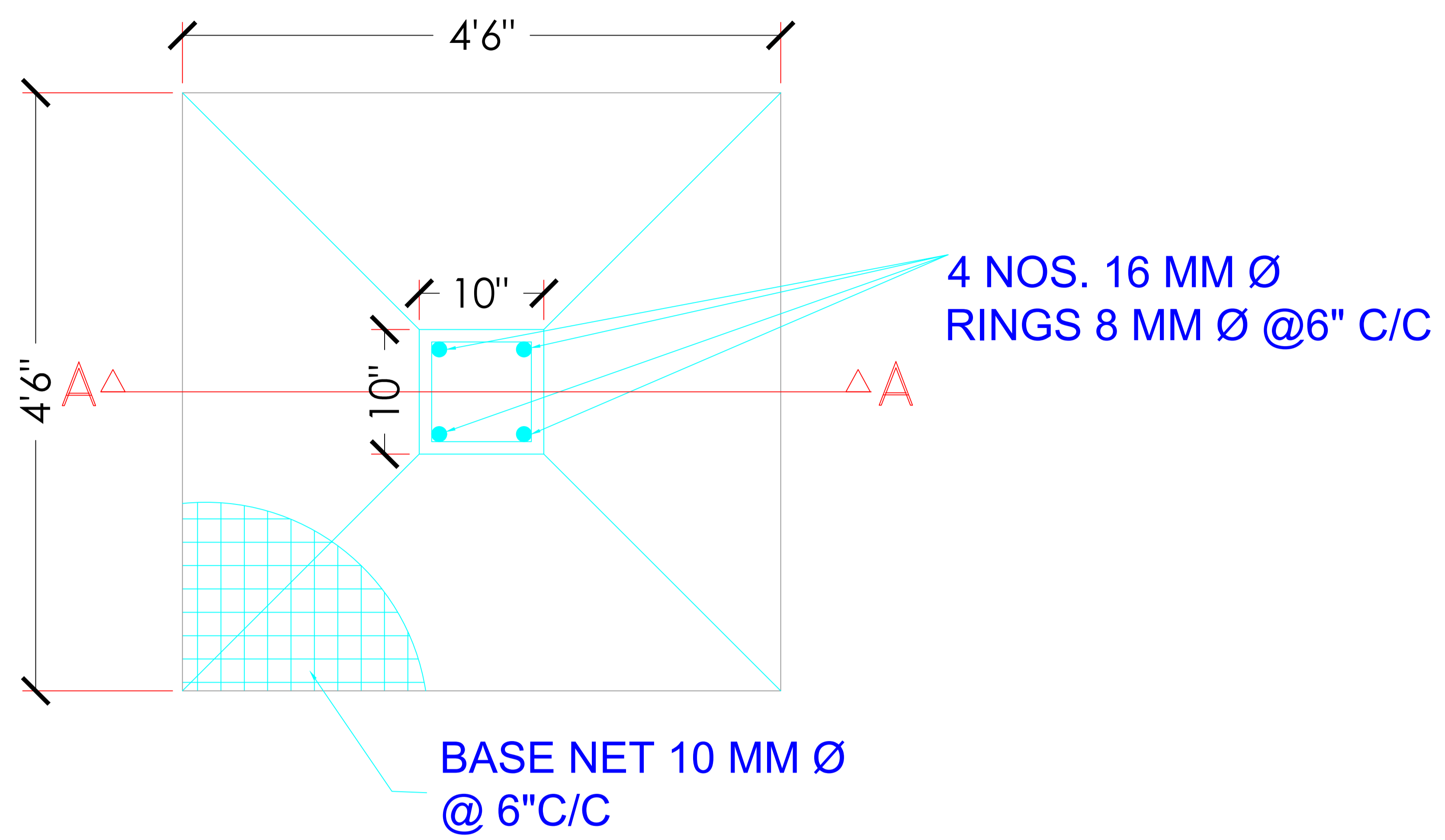
PLAN OF COLUMN FOUNDATION
