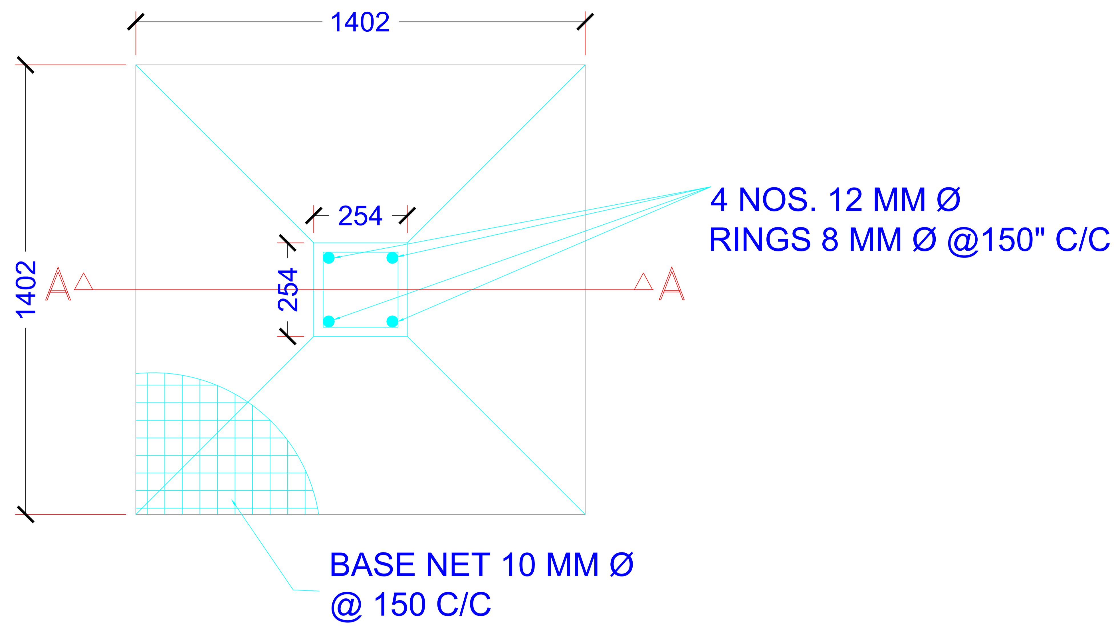
PLAN OF COLUMN FOUNDATION
