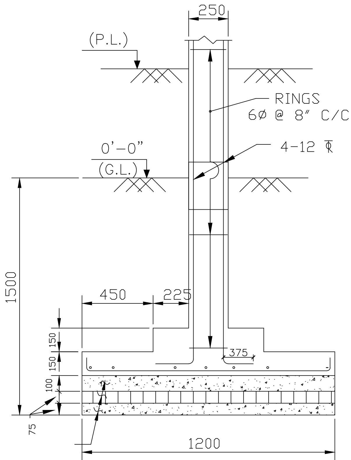
SECTION B-B
