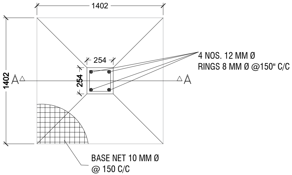
PLAN OF COLUMN FOUNDATION
