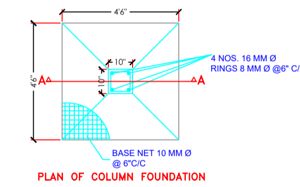
PLAN OF COLUMN FOUNDATION SCALE= 1:50
