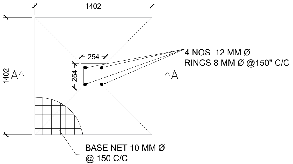
PLAN OF COLUMN FOUNDATION
