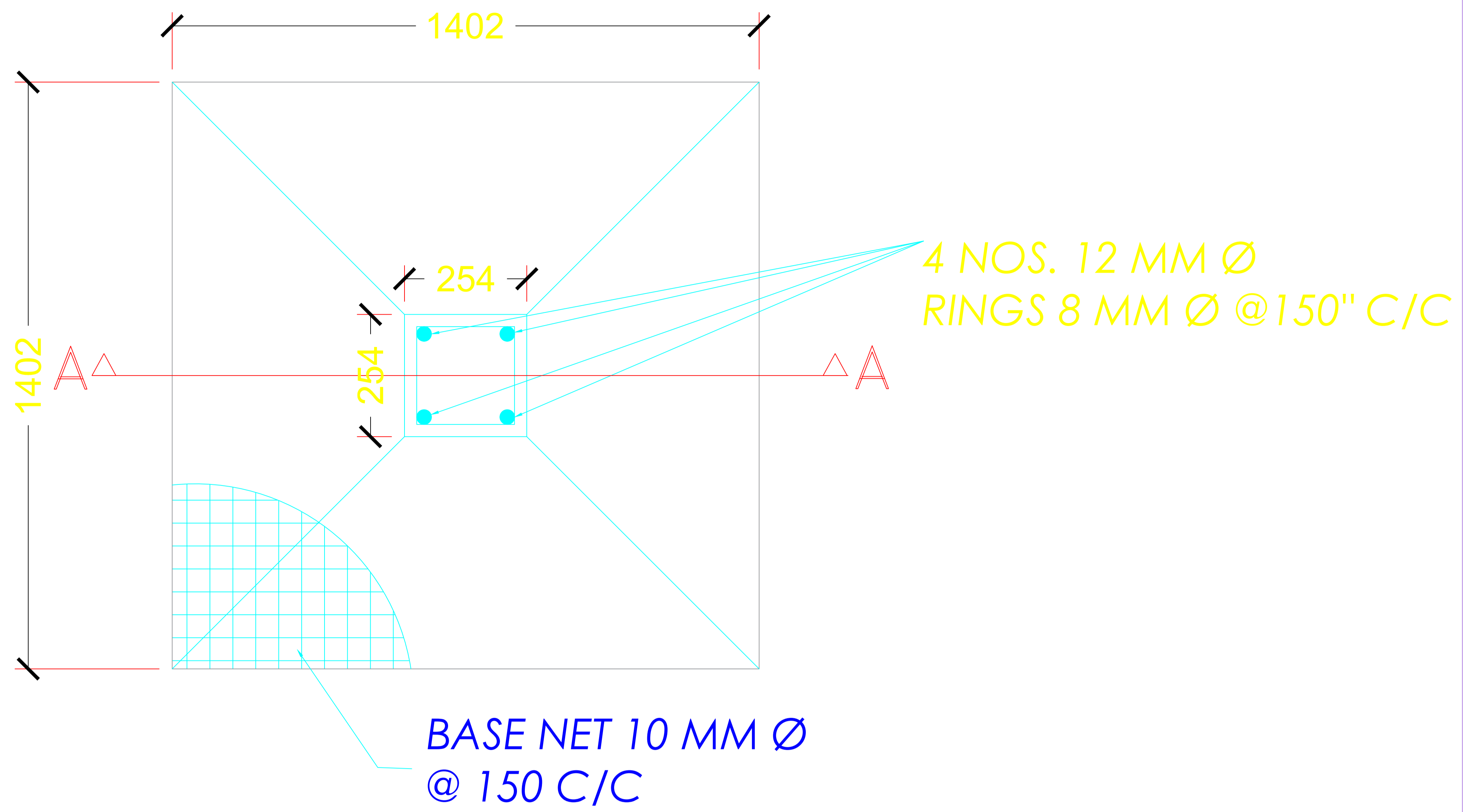
PLAN OF COLUMN FOUNDATION
