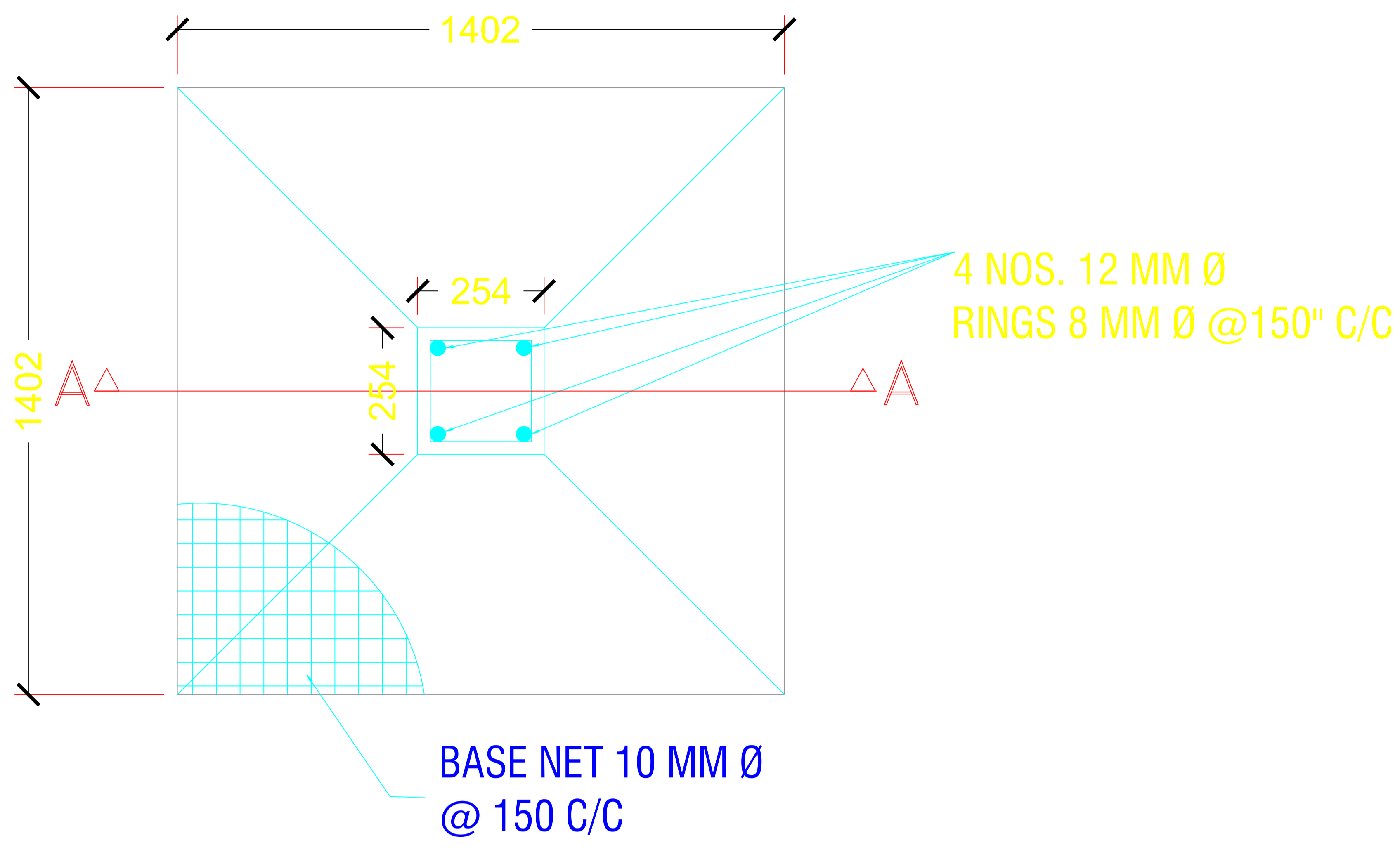
PLAN OF COLUMN FOUNDATION
