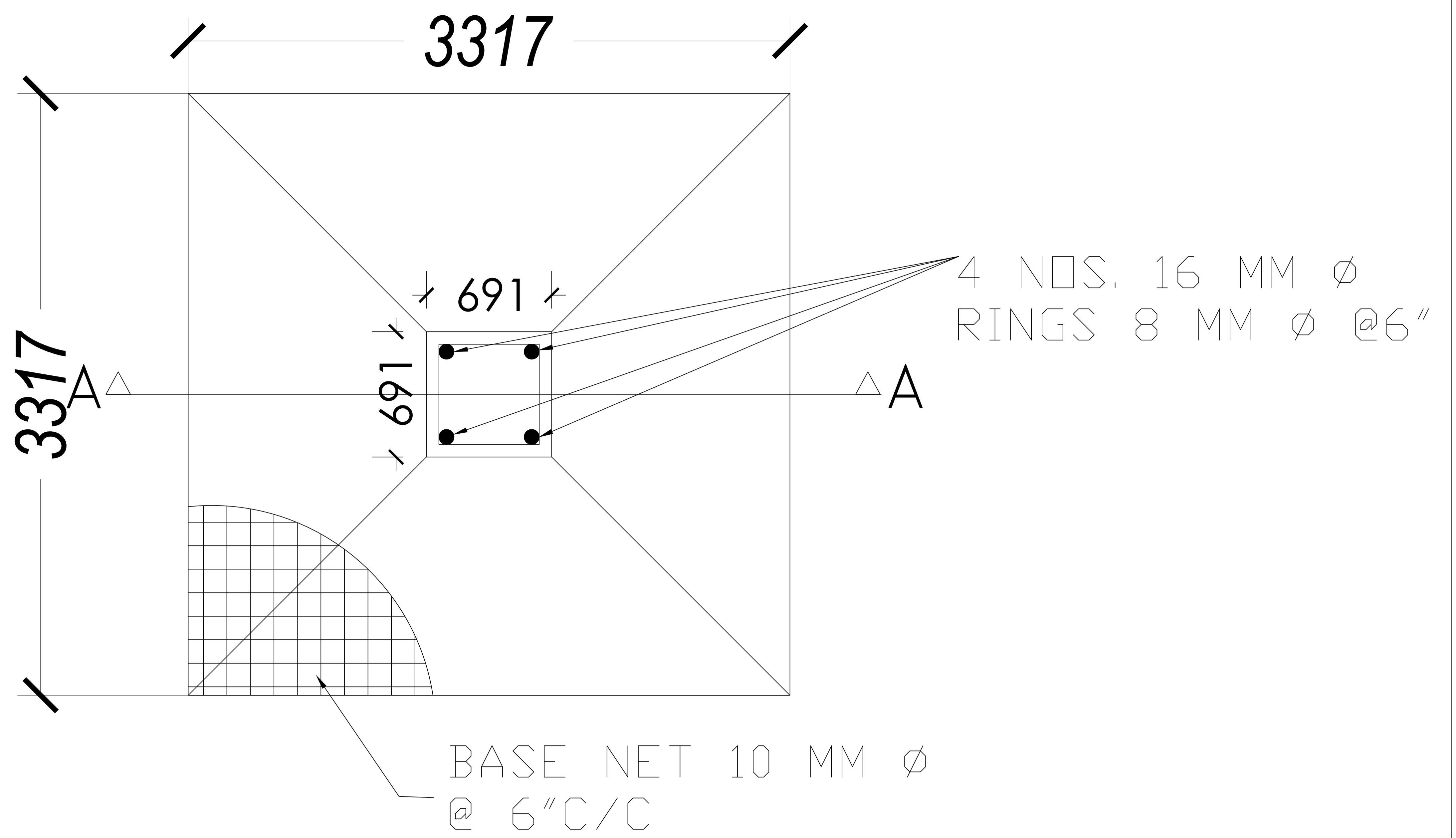
PLAN OF COLUMN FOUNDATION
