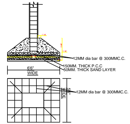
FOOTING CROSS SECTION DETAILS.
