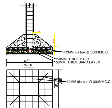
FOOTING CROSS SECTION DETAILS.
