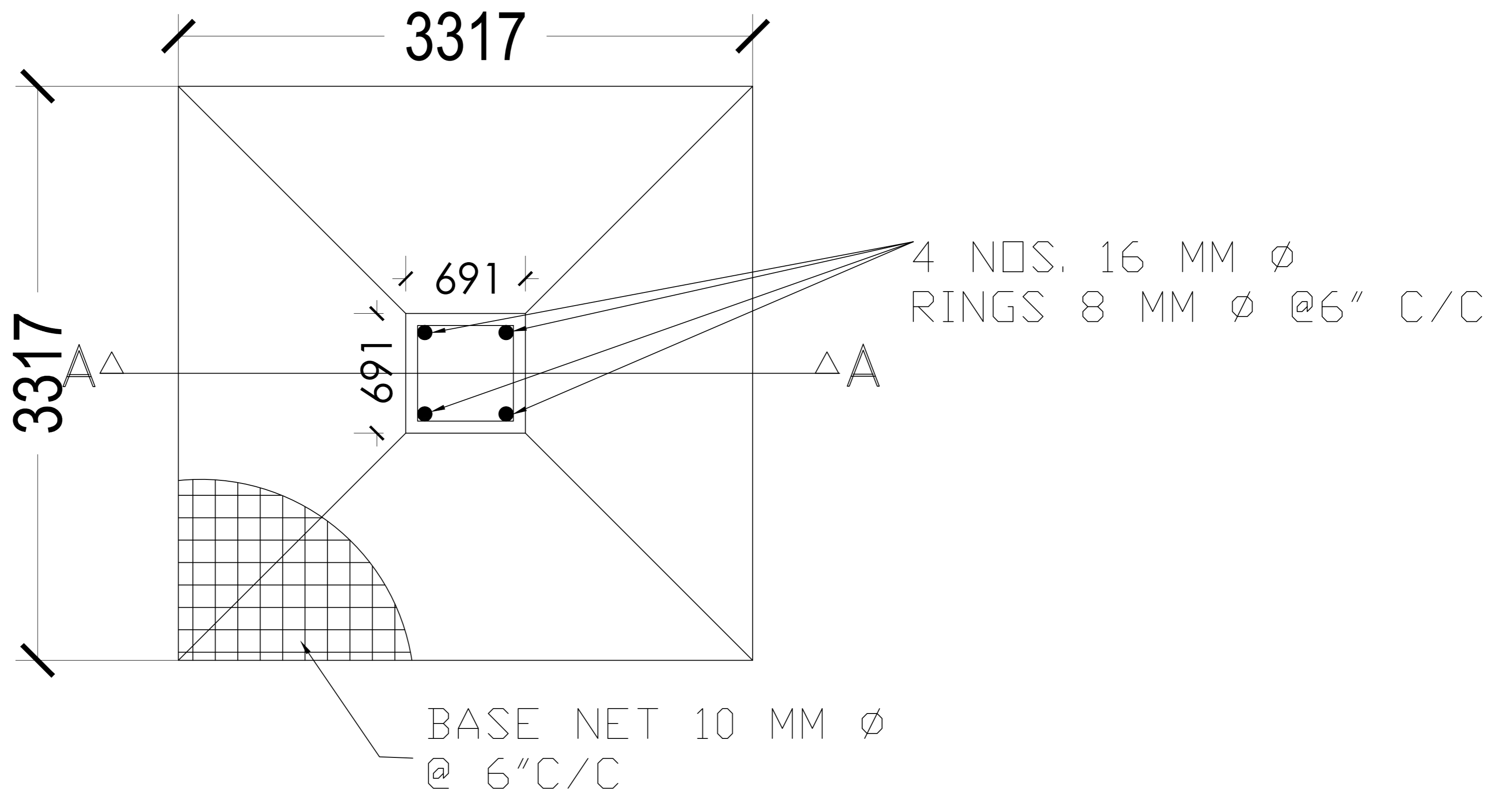
PLAN OF COLUMN FOUNDATION
