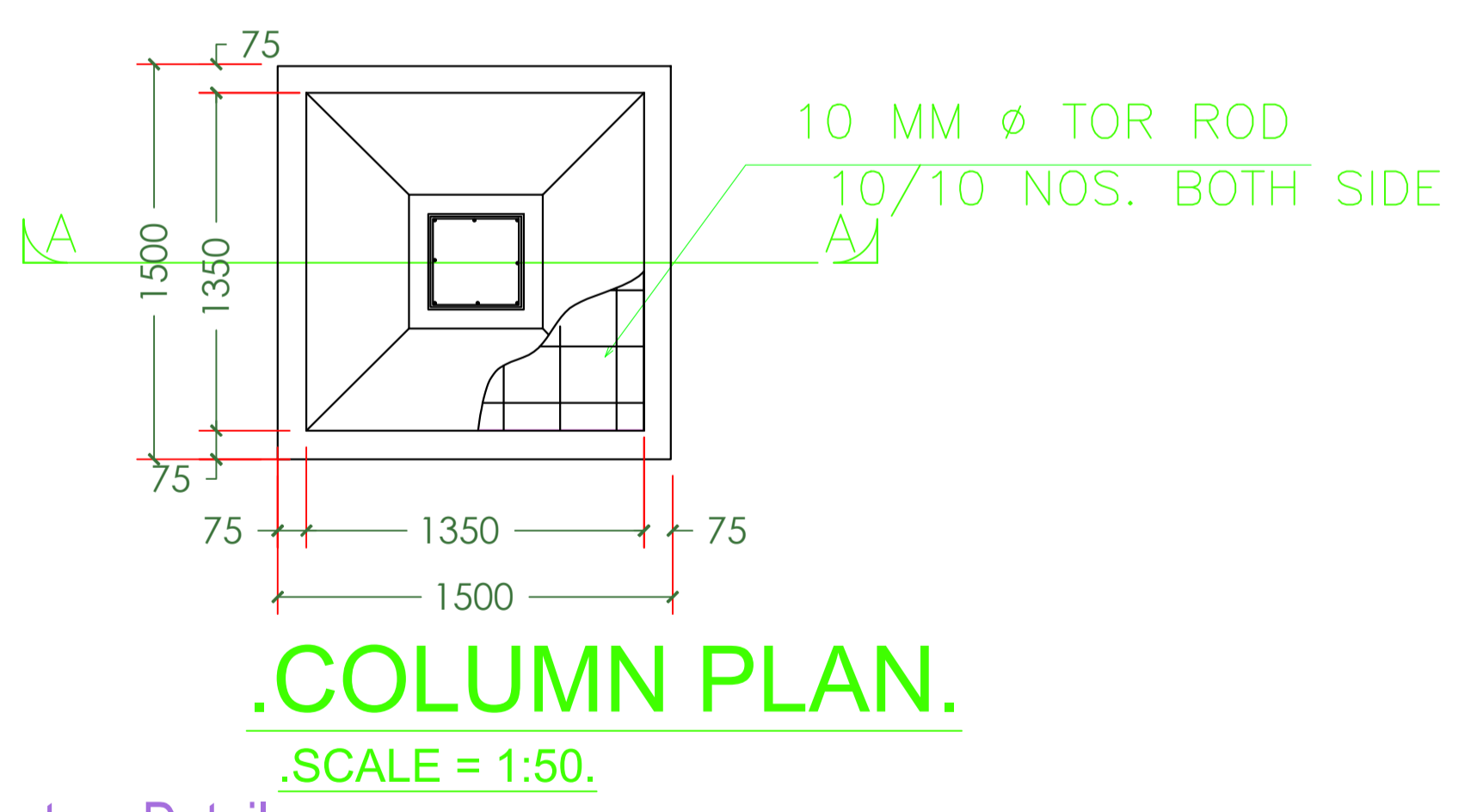
Structure Detail
