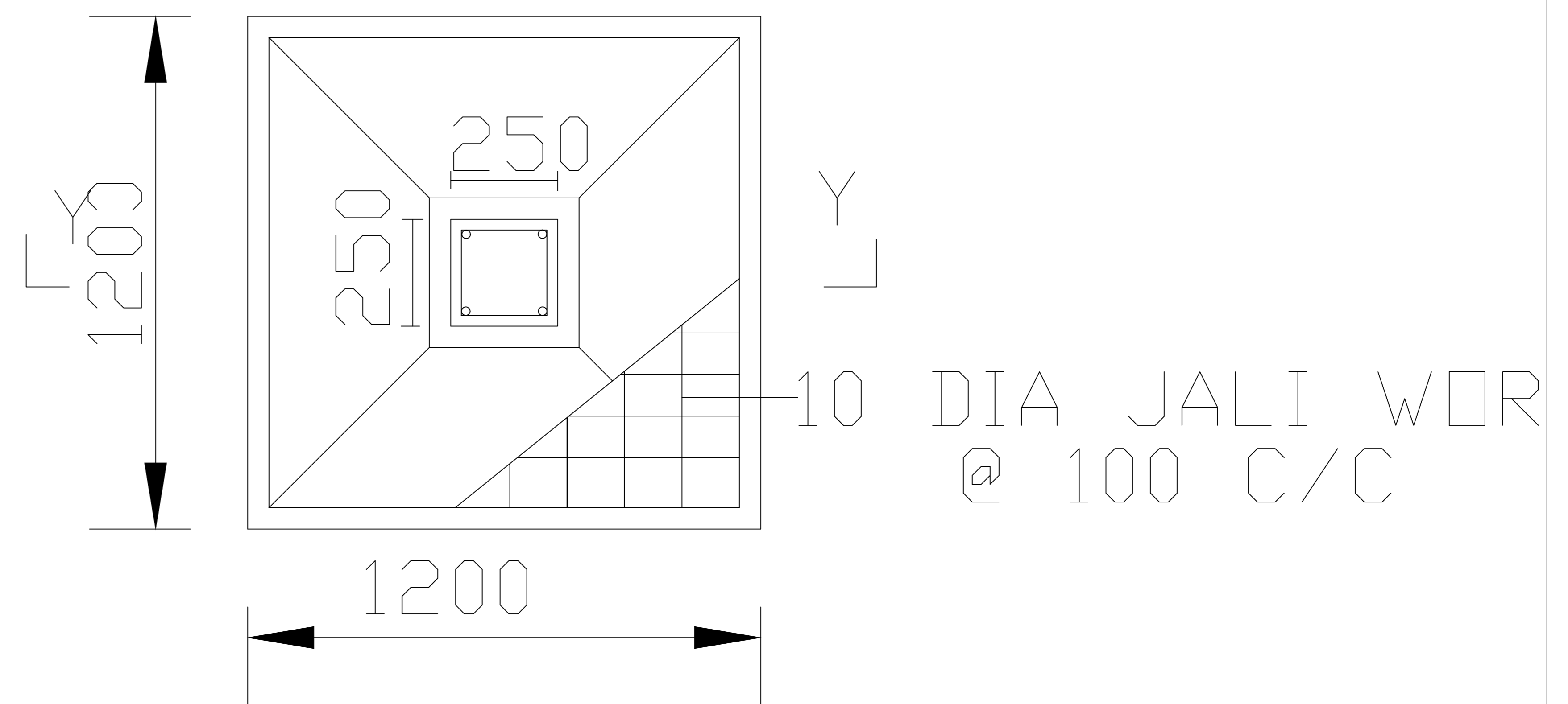
DETAIL OF FOUNDATION
