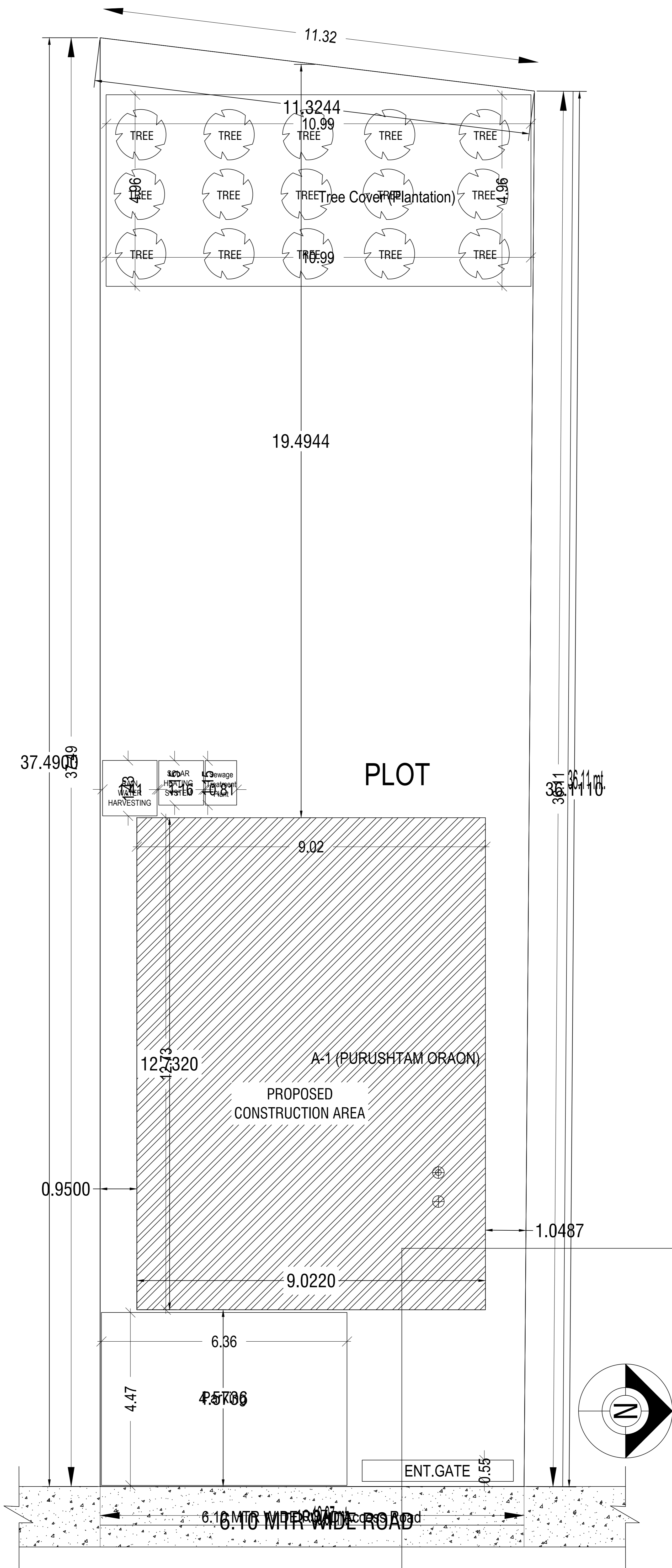
SITE PLAN
