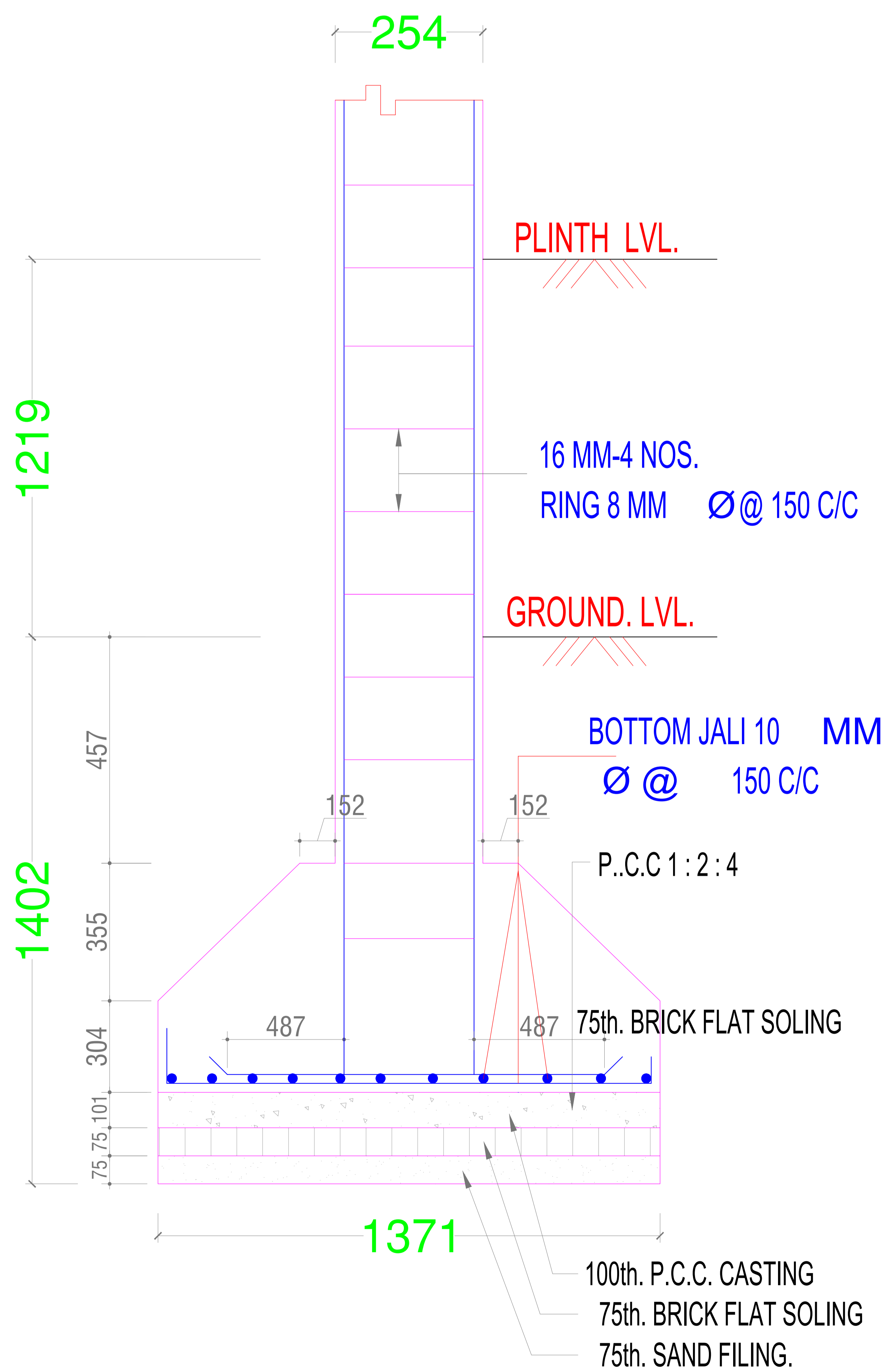
SECTION ON A-A
