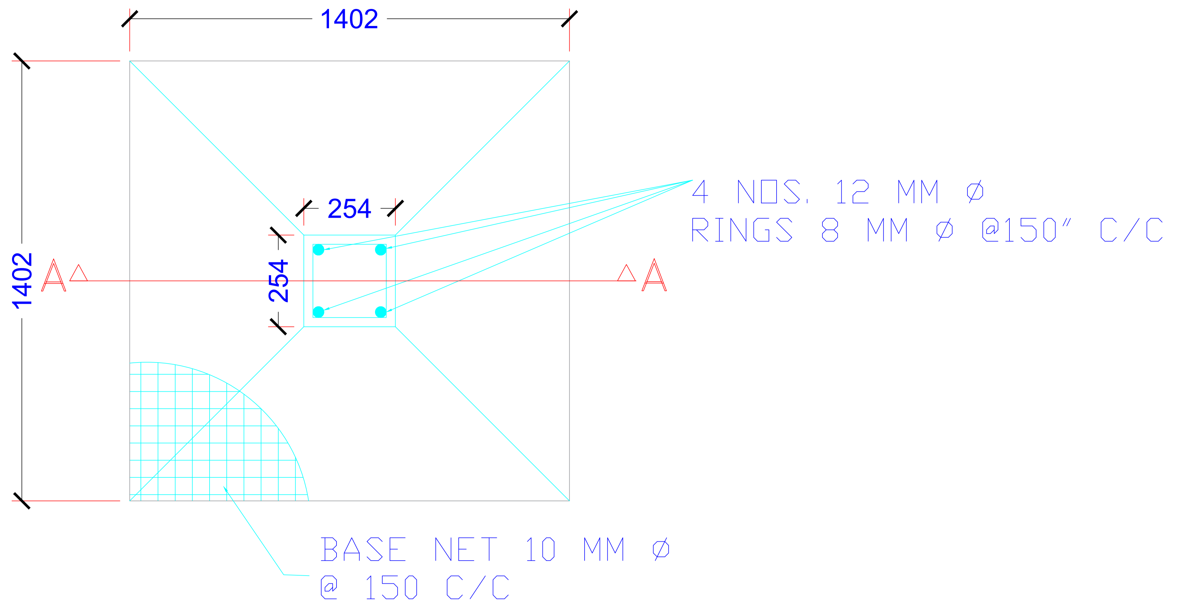
PLAN OF COLUMN FOUNDATION
