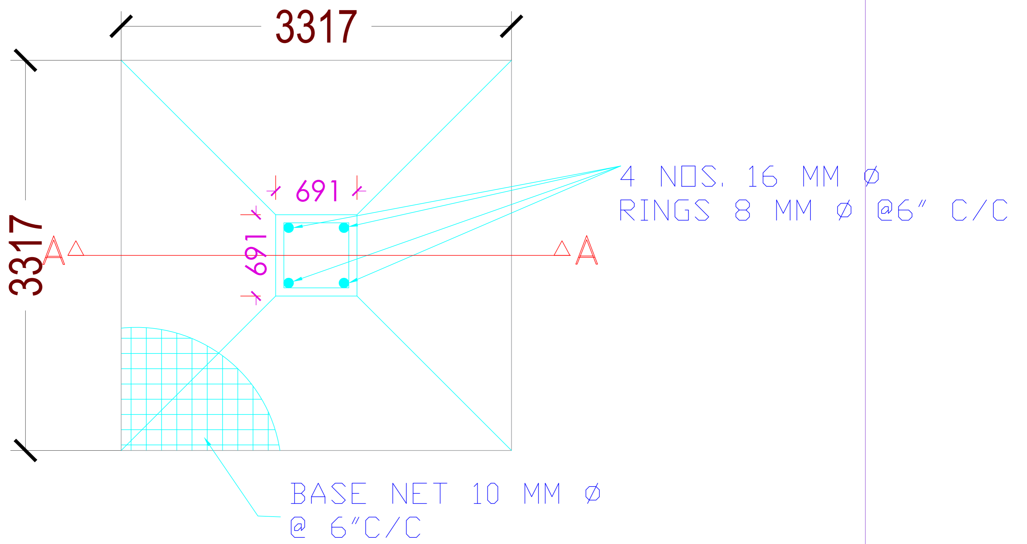
PLAN OF COLUMN FOUNDATION
