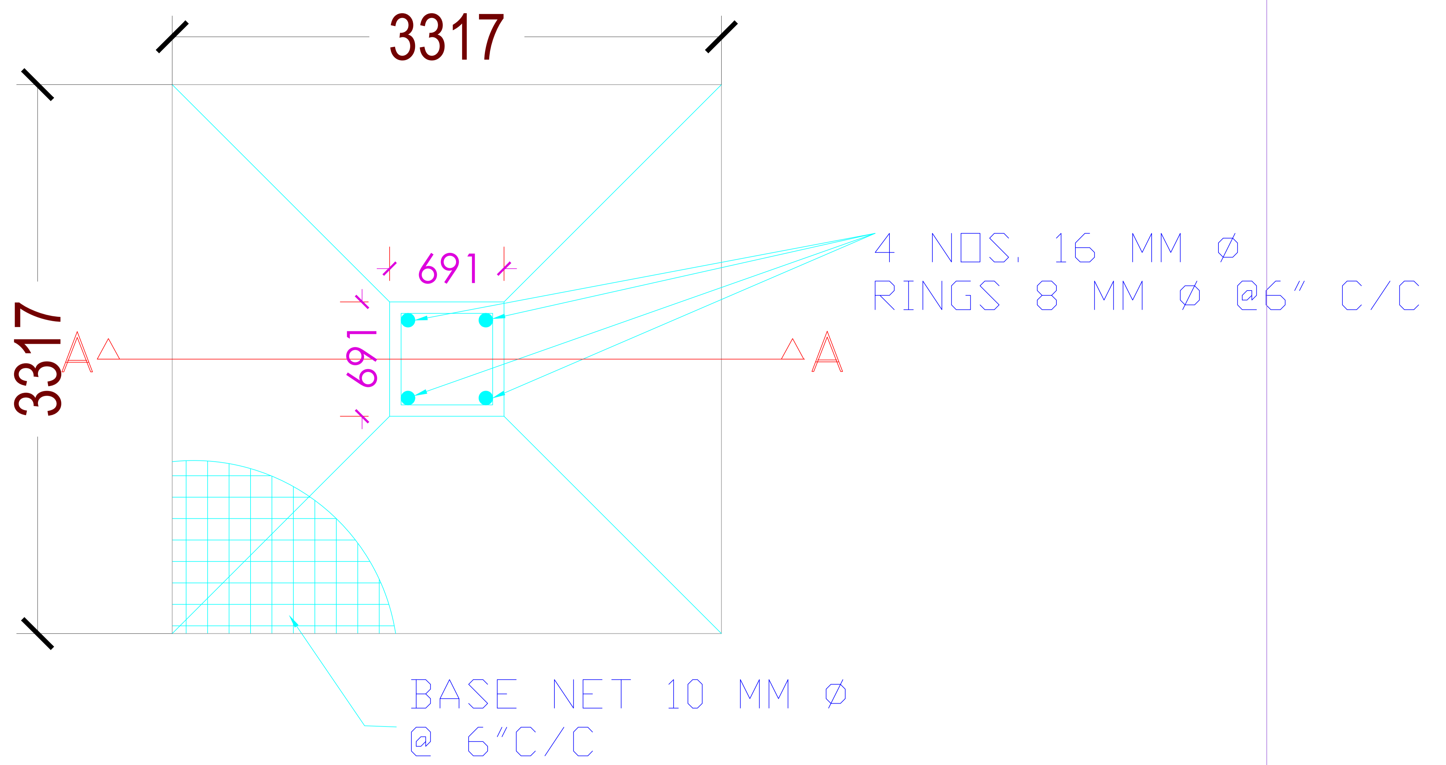
PLAN OF COLUMN FOUNDATION
