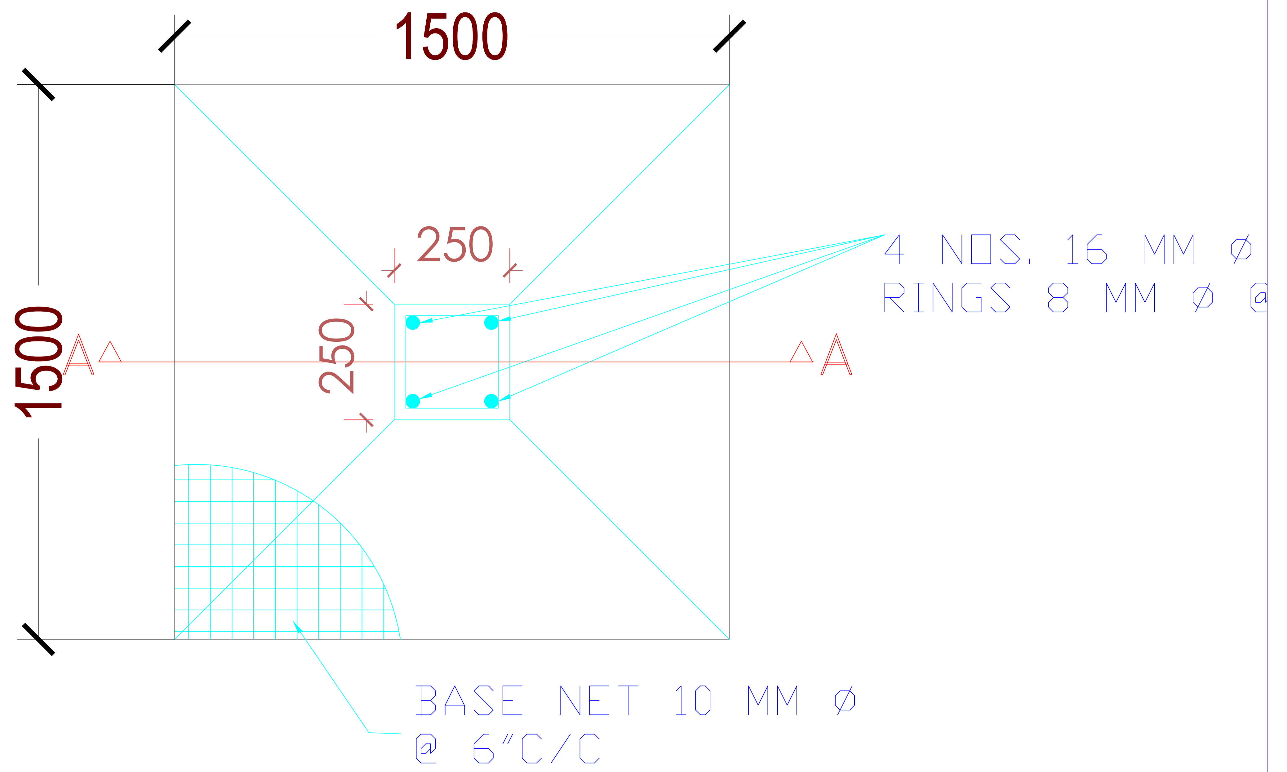
PLAN OF COLUMN FOUNDATION
