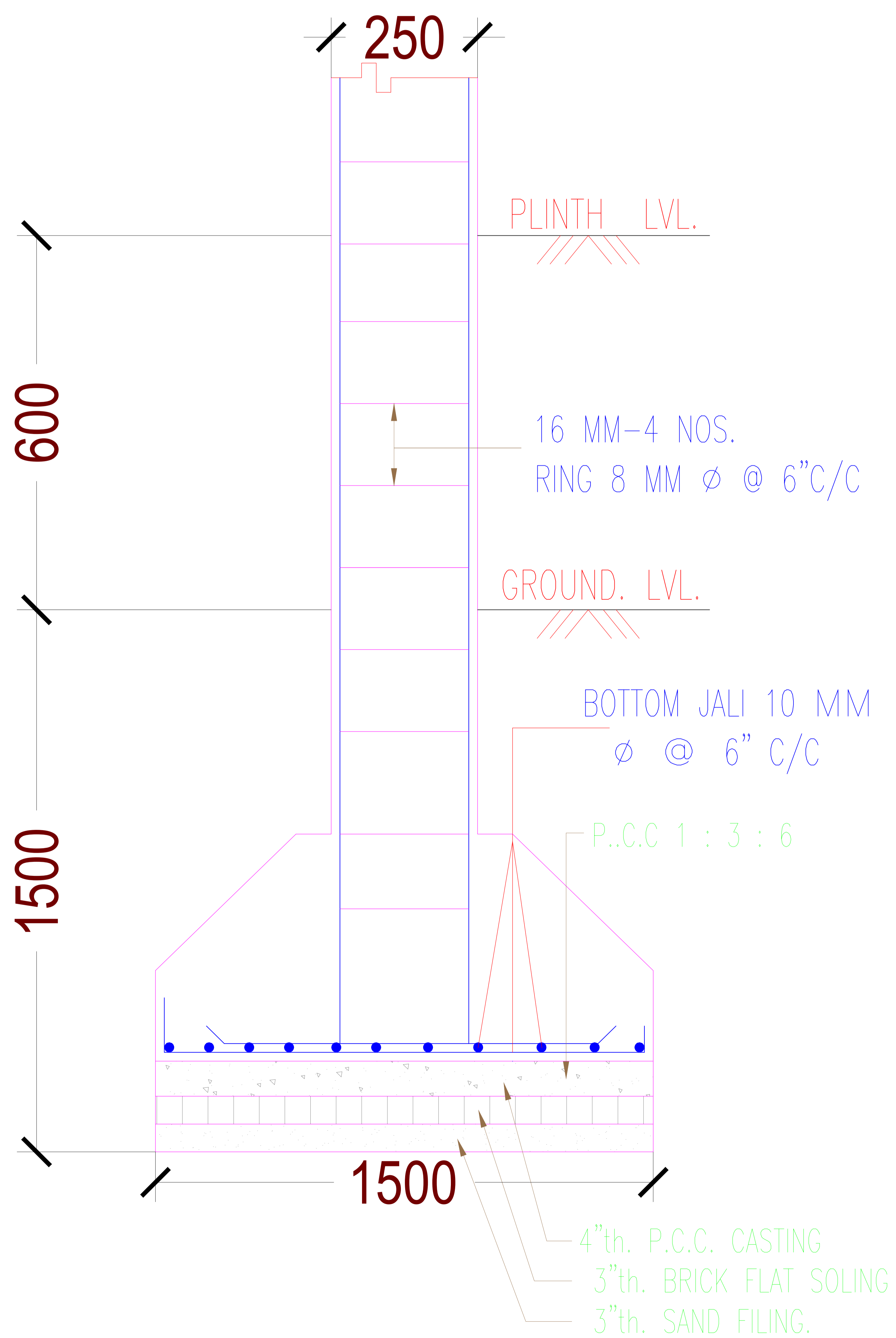
SECTION ON A-A
