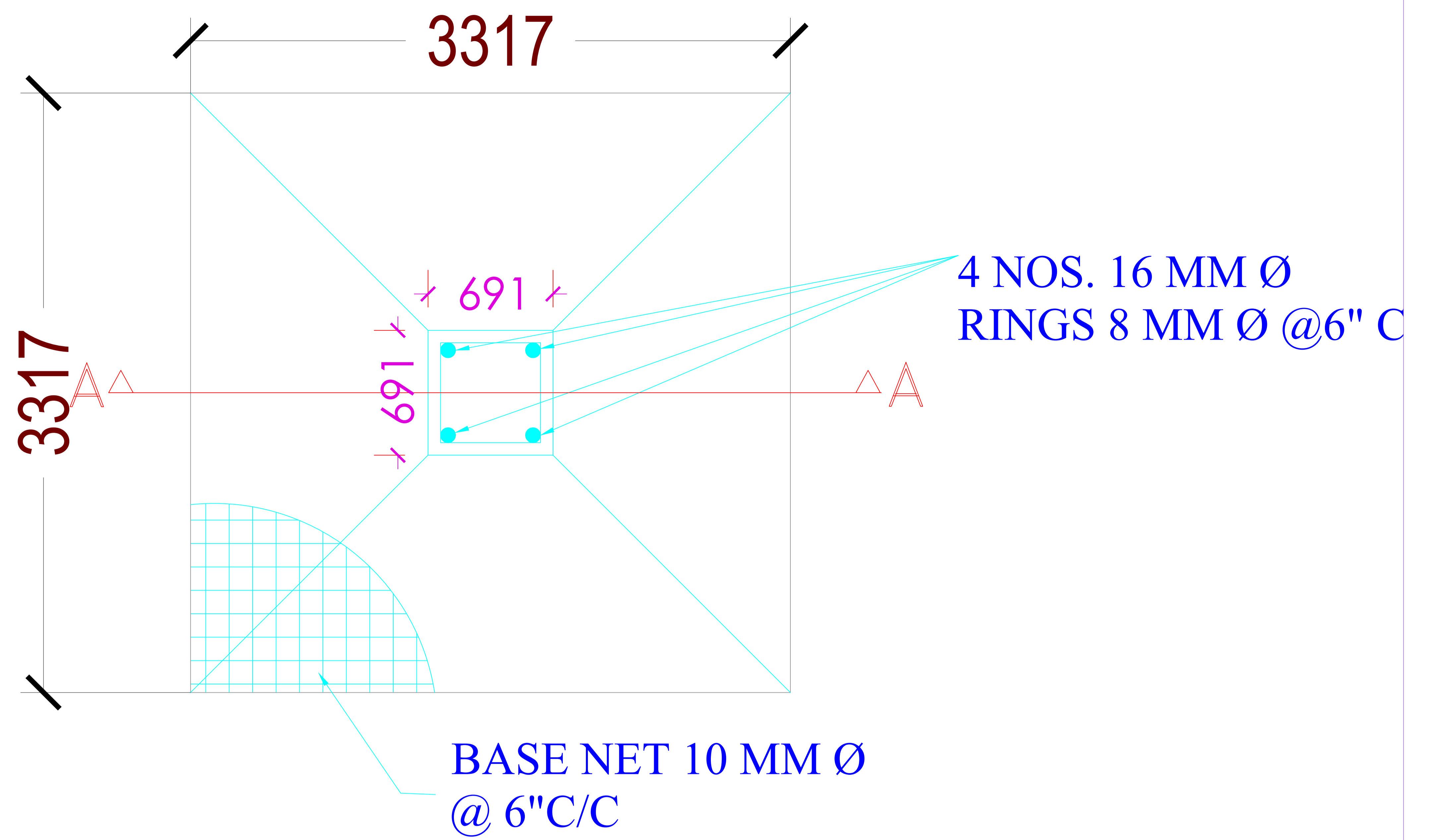
PLAN OF COLUMN FOUNDATION
