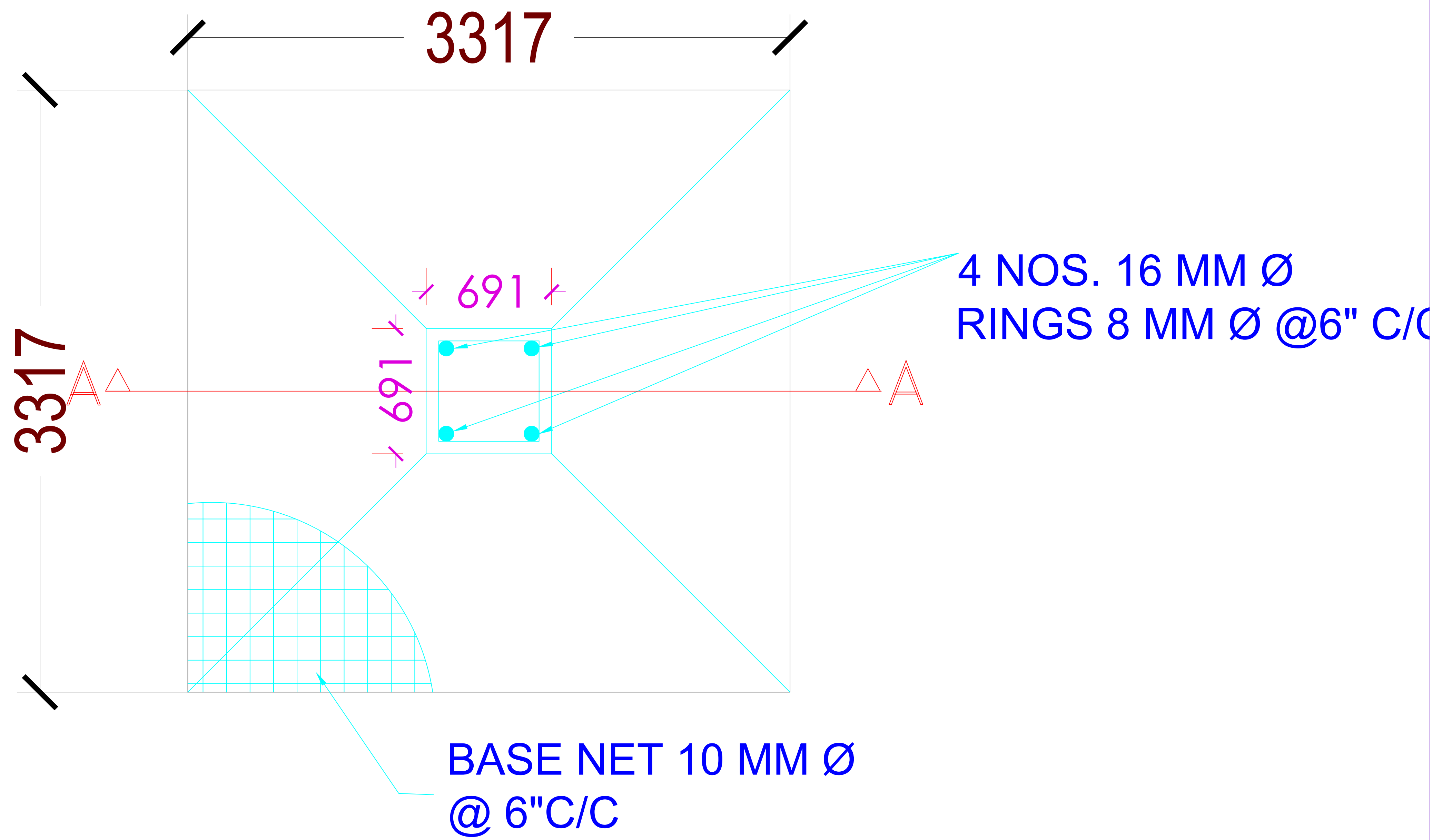
PLAN OF COLUMN FOUNDATION
