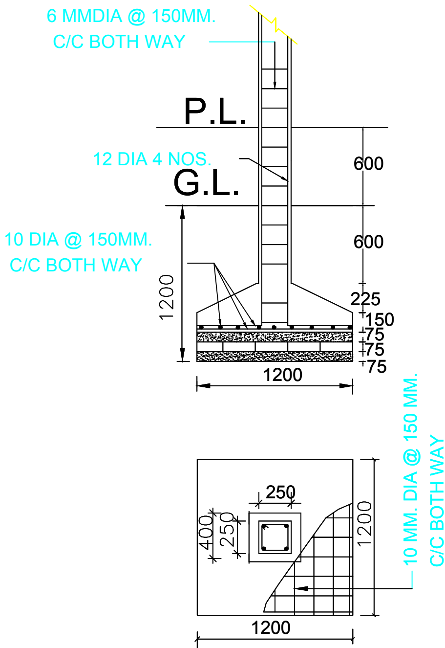
DETAILS OF R.C.C. COLUMN SCALE :- 1:50
