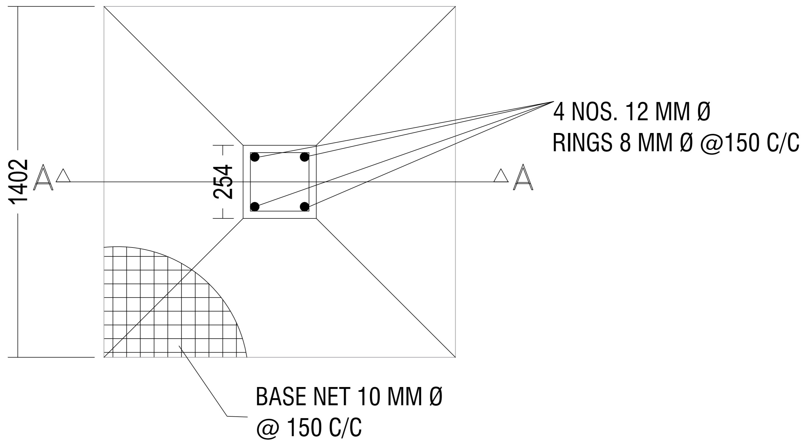
PLAN OF COLUMN FOUNDATION
