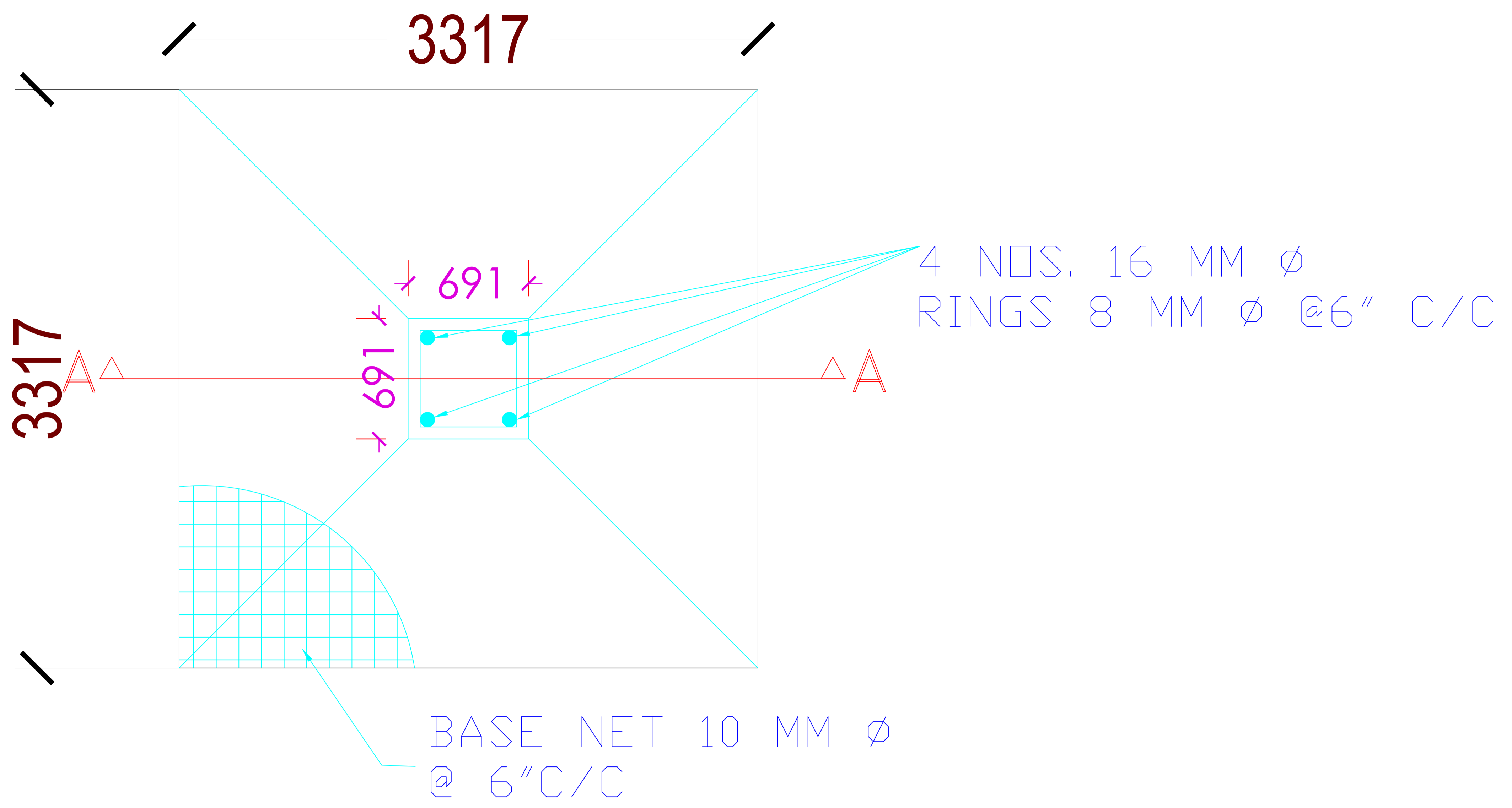
PLAN OF COLUMN FOUNDATION
