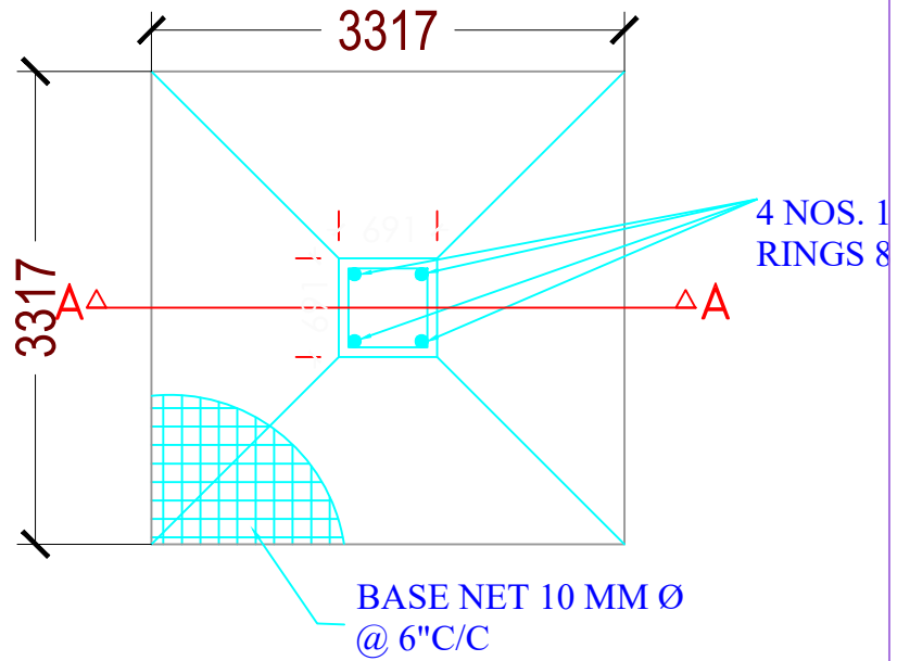
PLAN OF COLUMN FOUNDATION
