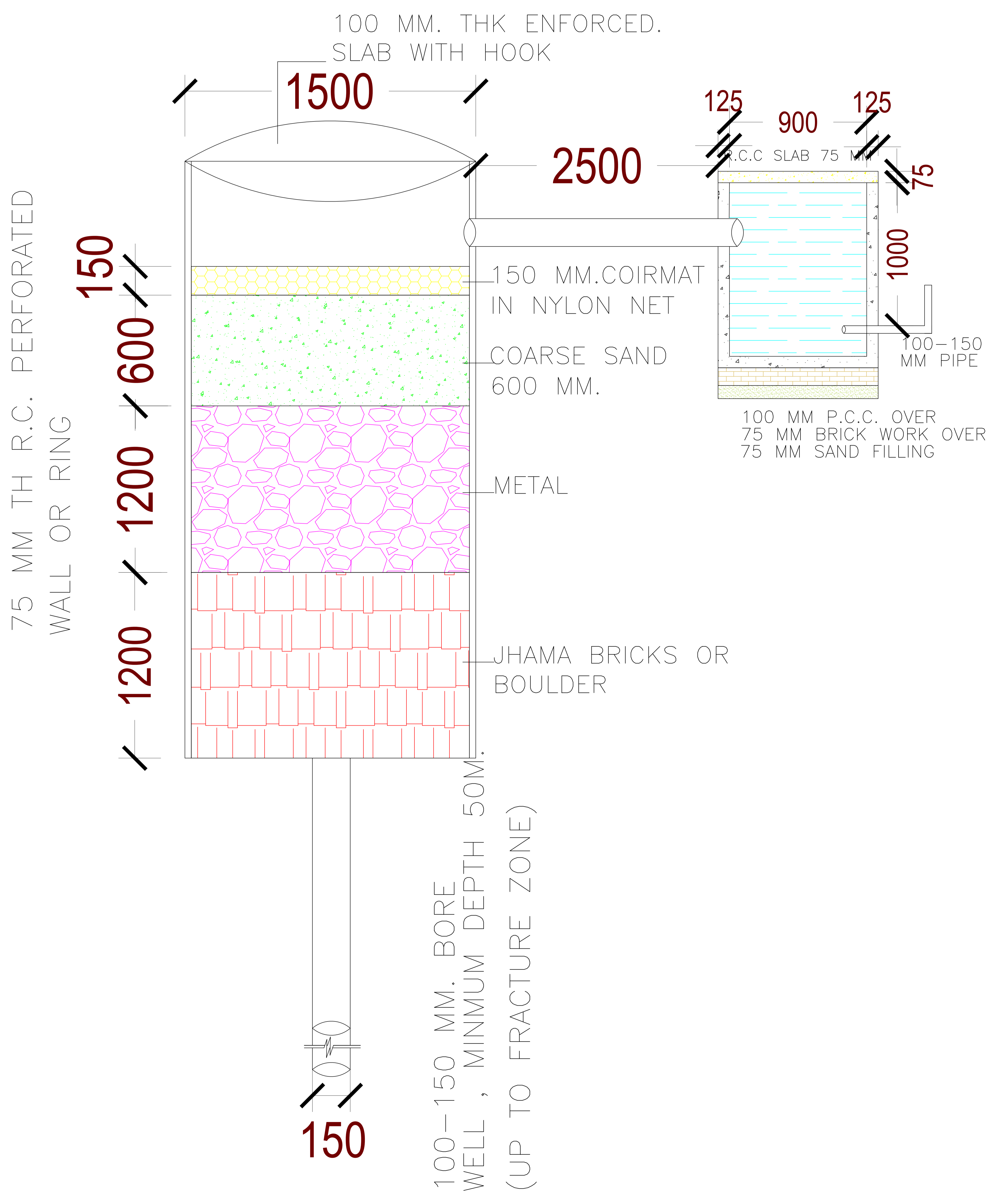
SECTION AT A-A (SCALE 1:50)
