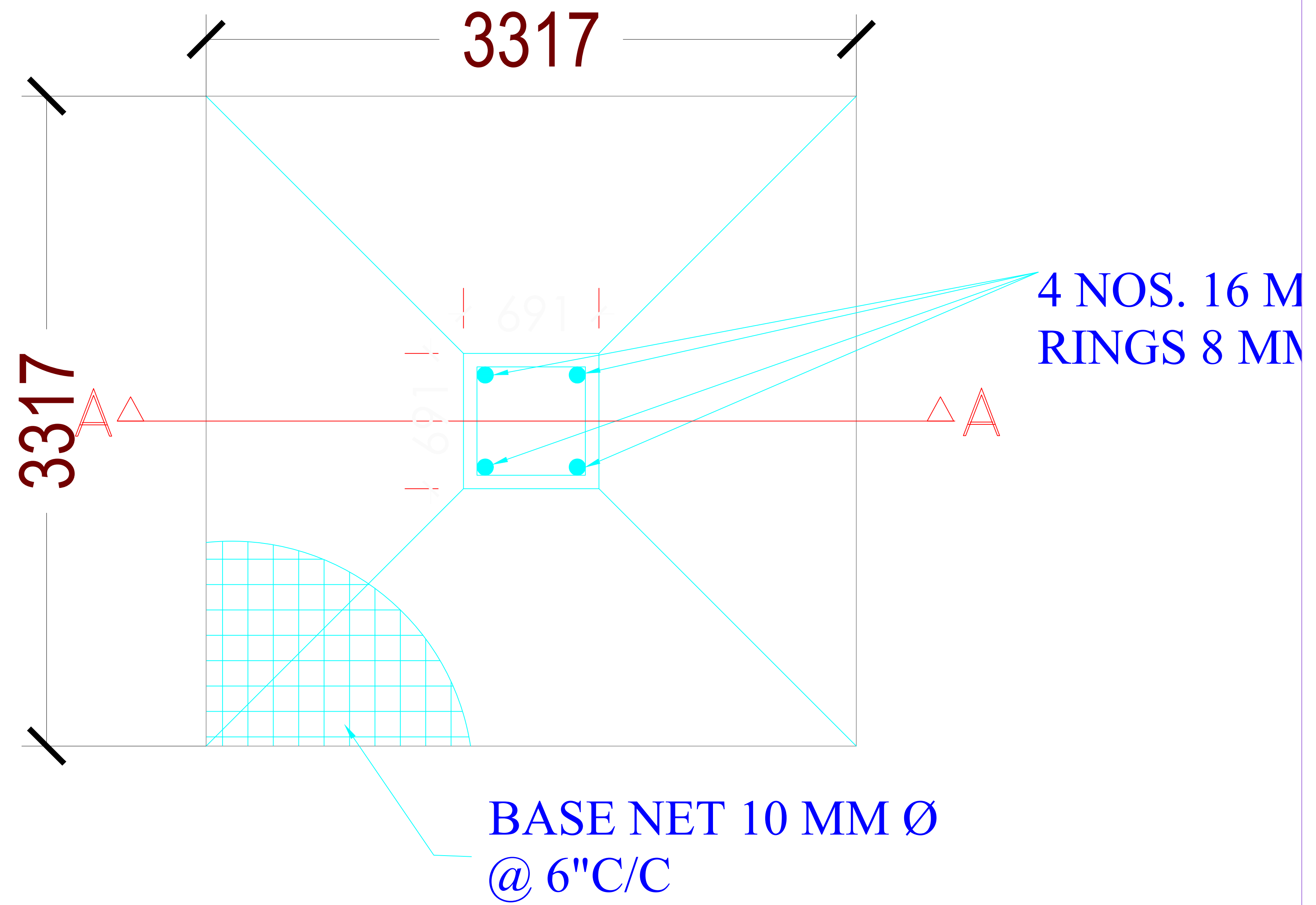
PLAN OF COLUMN FOUNDATION
