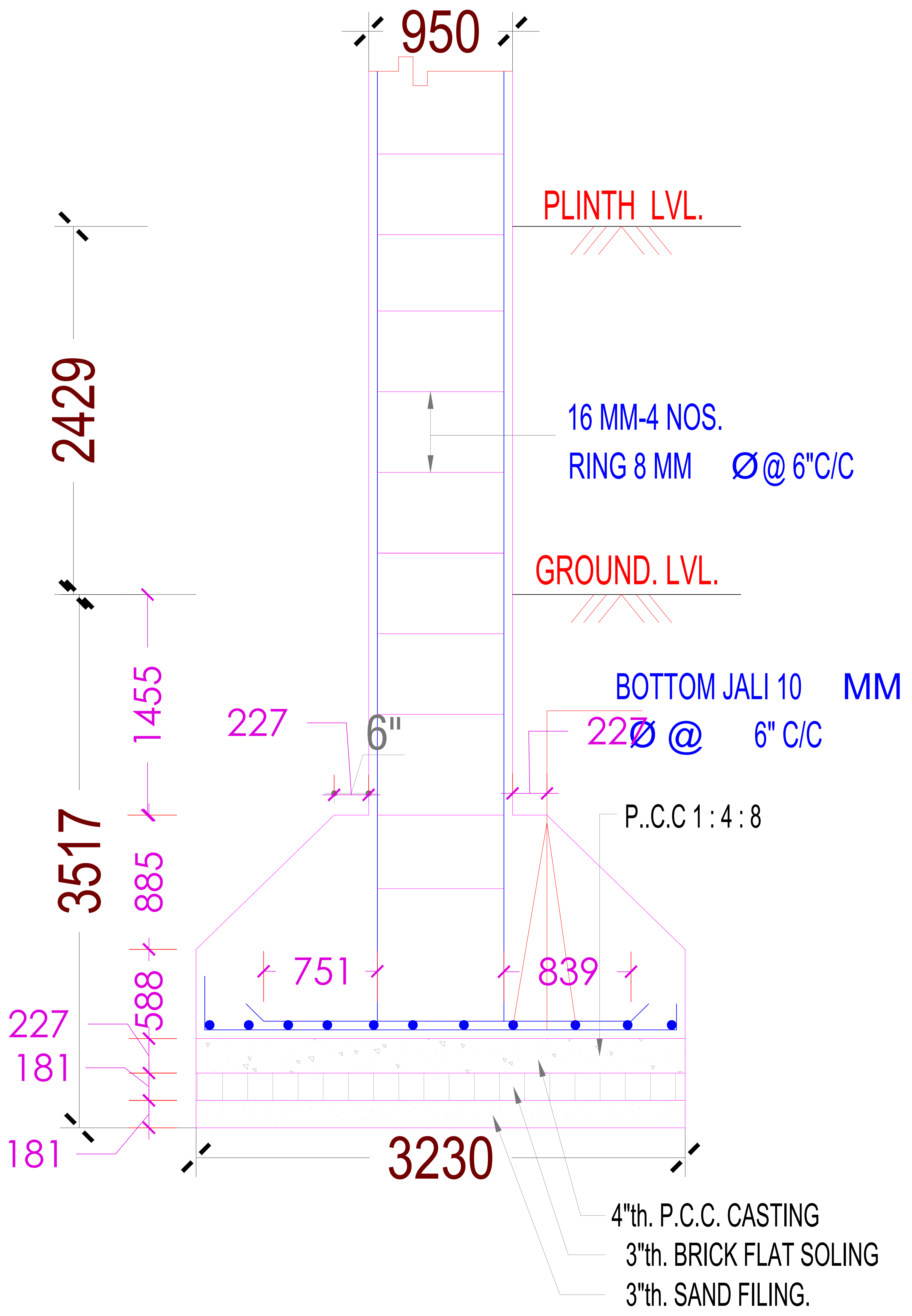
SECTION ON A-A SCALE= 1:50
