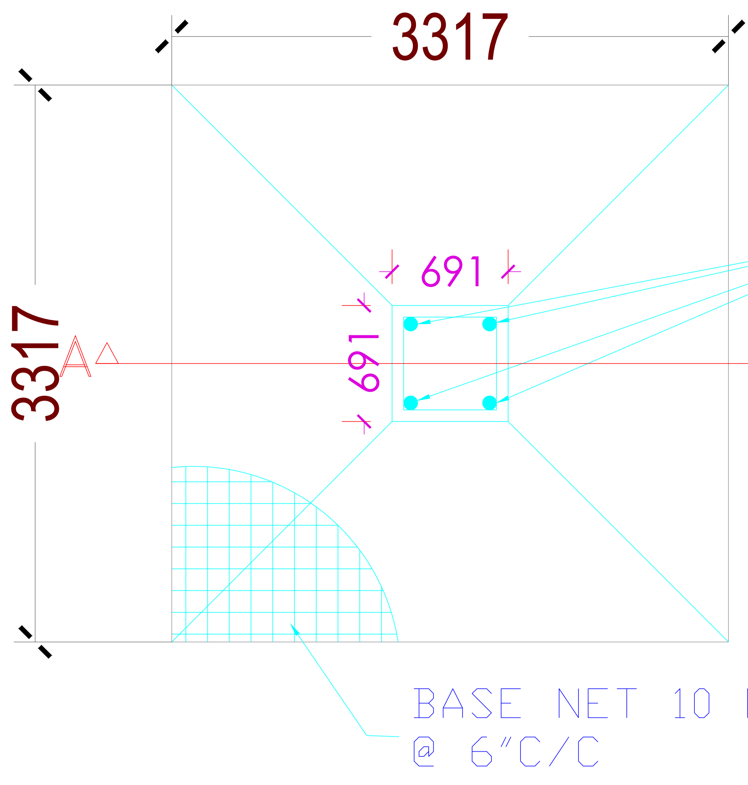
PLAN OF COLUMN FOUNDATION SCALE= 1:50
