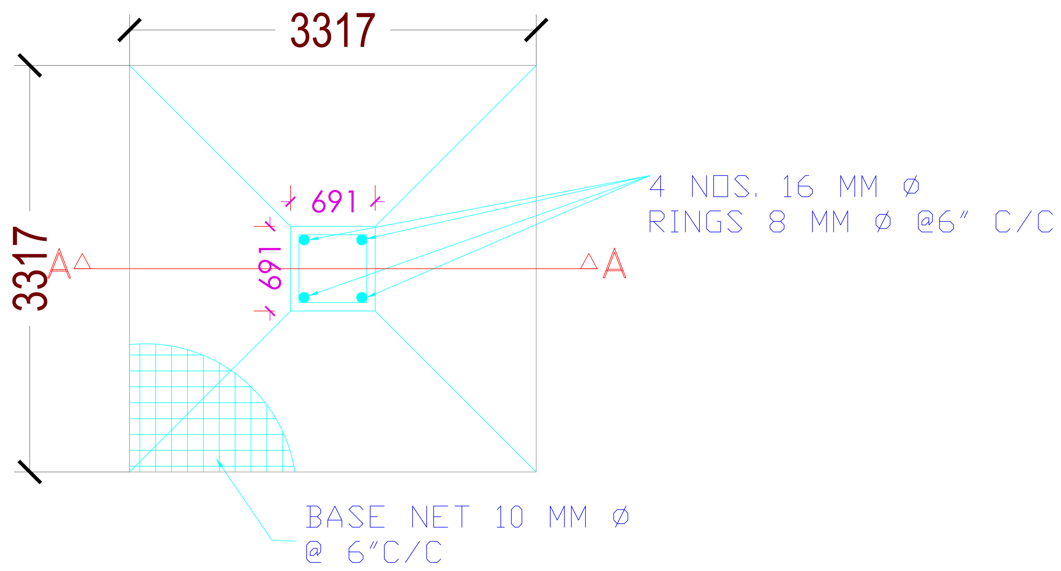
PLAN OF COLUMN FOUNDATION
