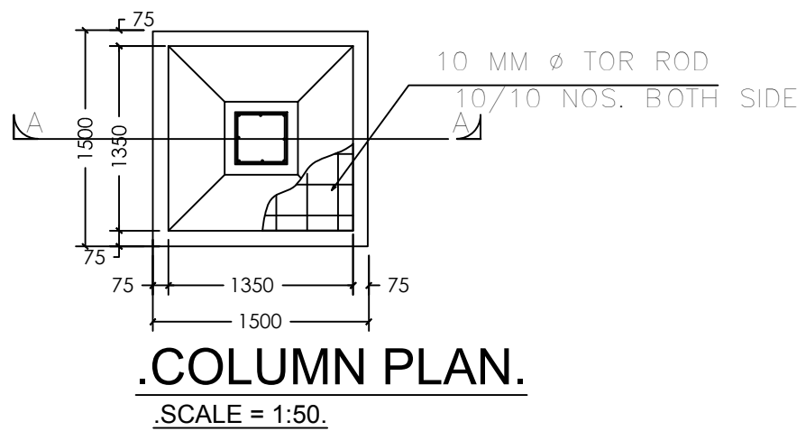
Structure Detail
