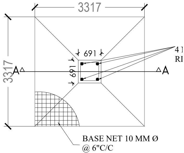
PLAN OF COLUMN FOUNDATION
