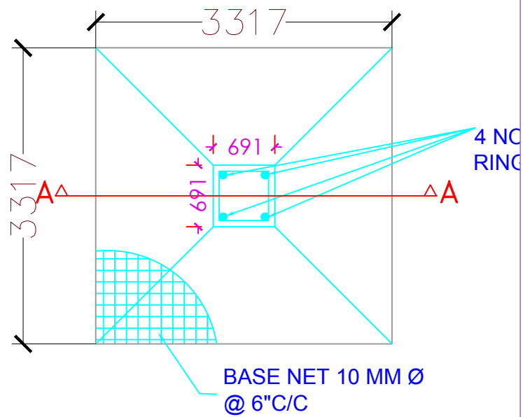
PLAN OF COLUMN FOUNDATION
