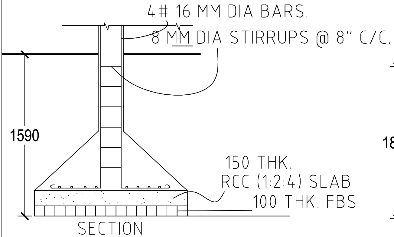
FOUNDATION DETAILS (ISOLATED R.C.C FOOTING)
