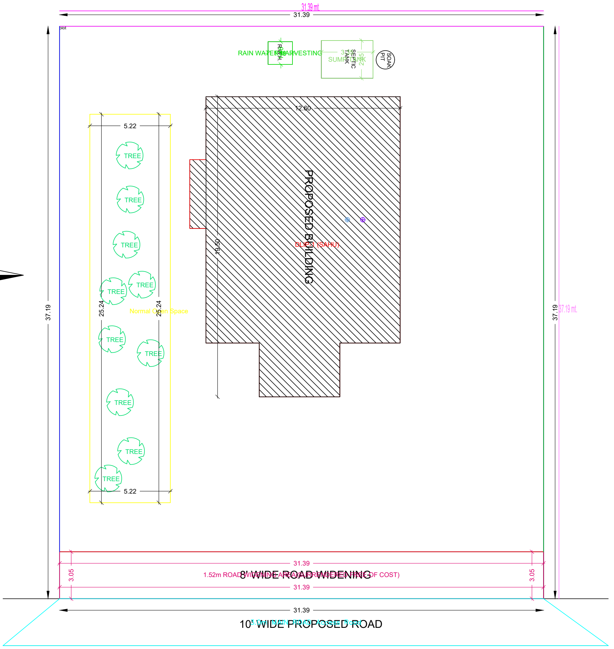
site plan
