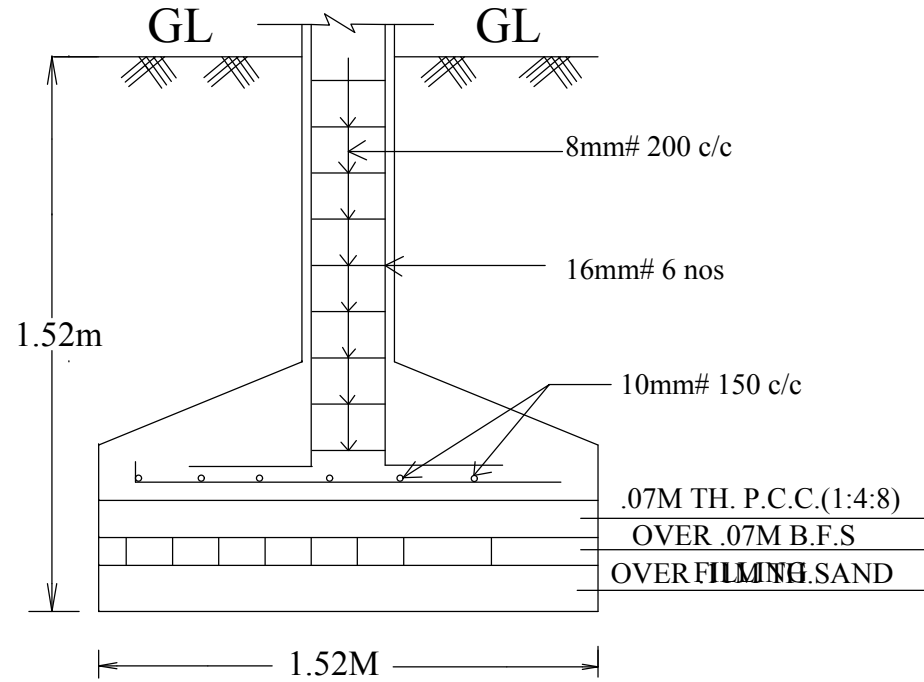
SECTION AT PP
