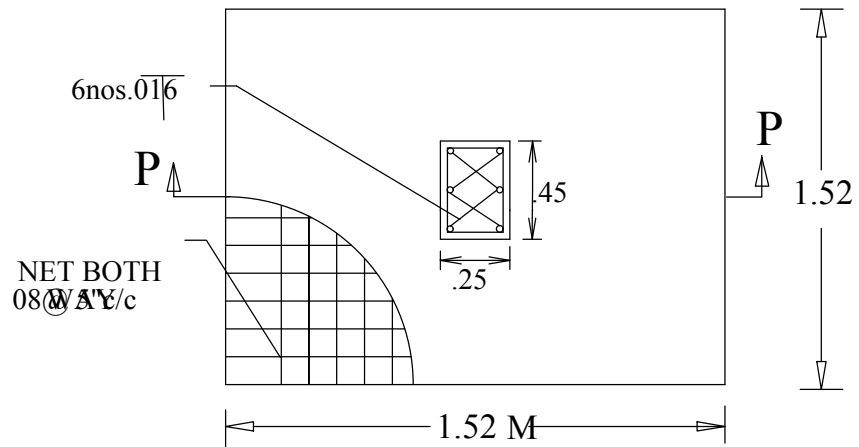
DETAIL OF R.C.C COL.
