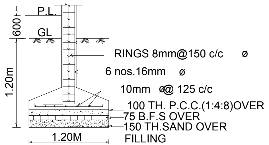
SECTION AT PP (NOT TO SCALE)
