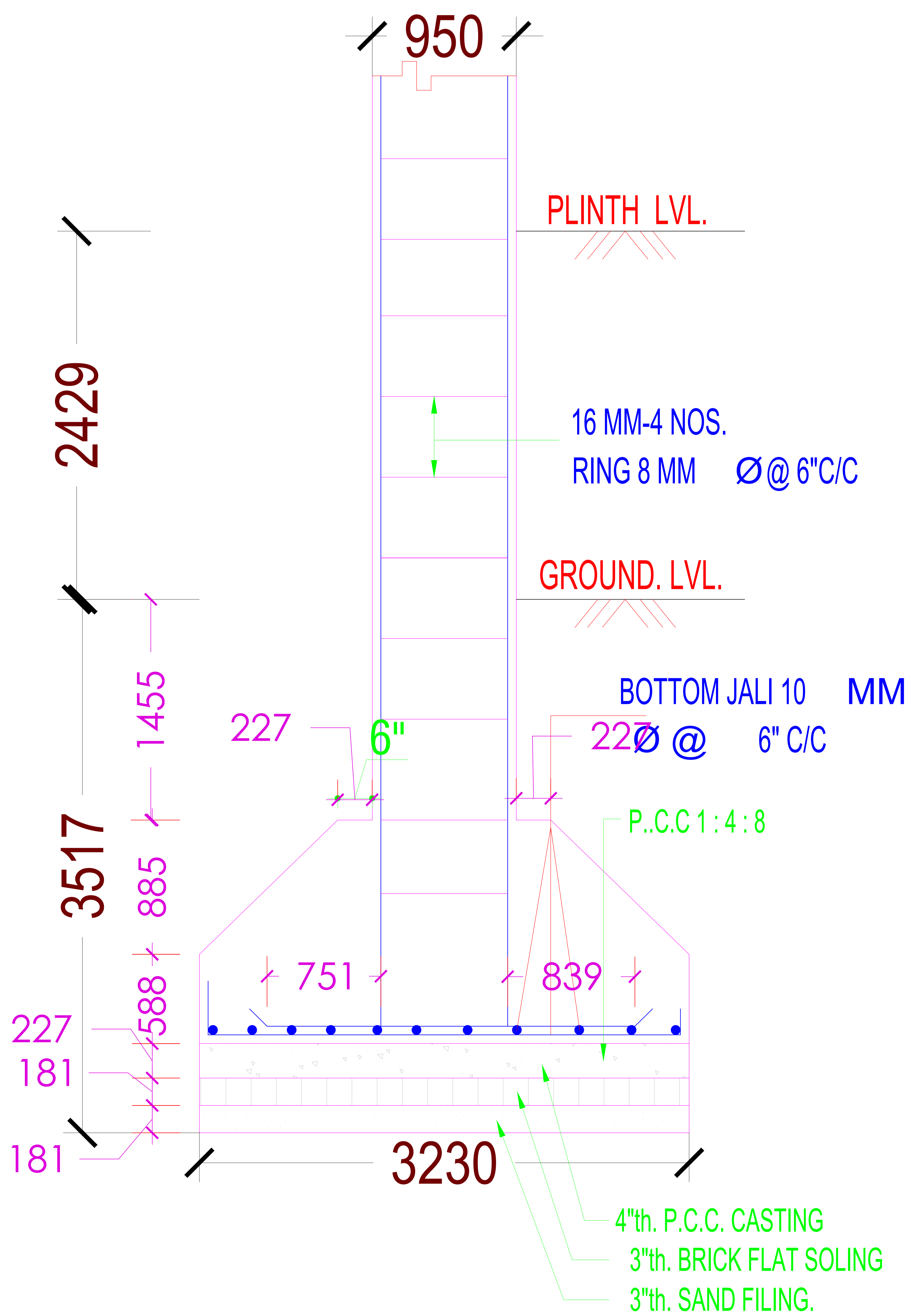
SECTION ON A-A
