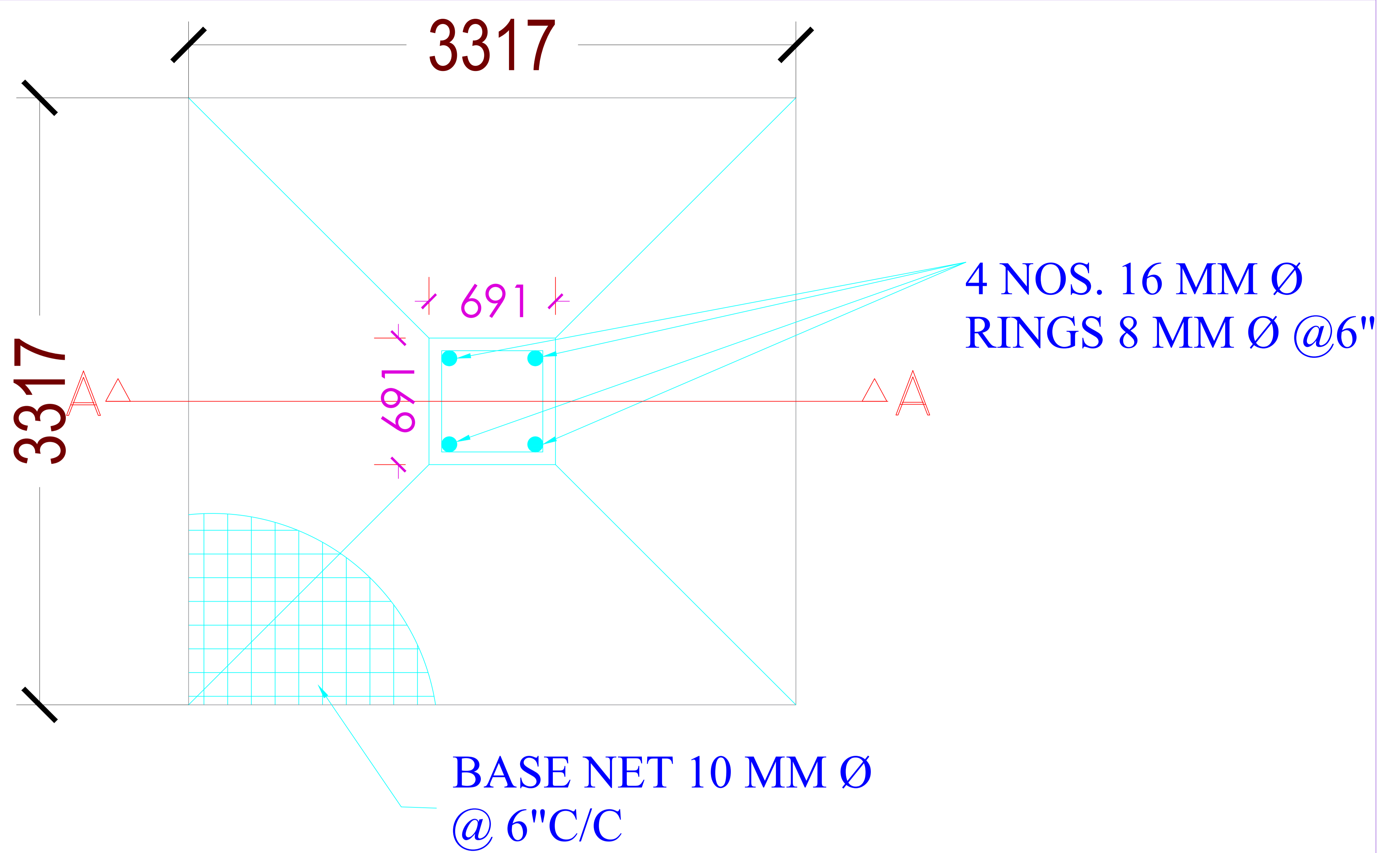
PLAN OF COLUMN FOUNDATION
