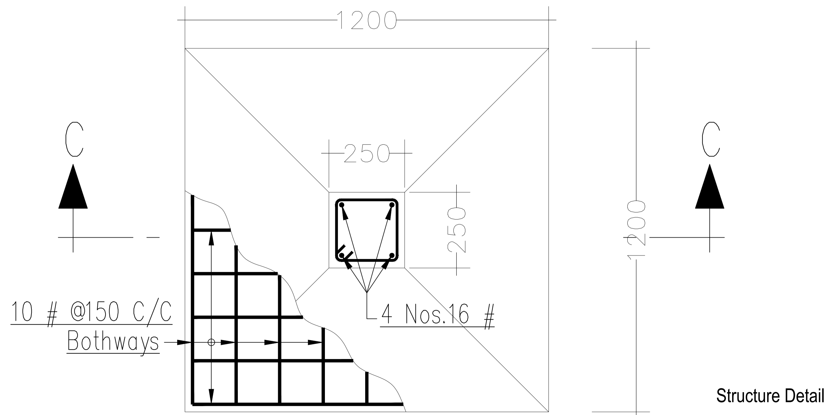
Typ. RCC (250X250) Column Details
