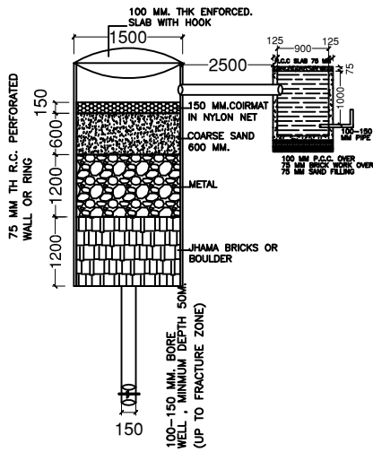
SECTION AT A-A (SCALE 1:50)
