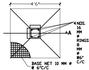
PLAN OF COLUMN FOUNDATION
