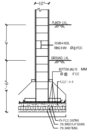
SECTION ON A-A
