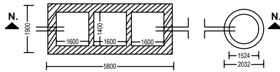
DETAIL OF SEPTIC TANK & SOAKPIT.
