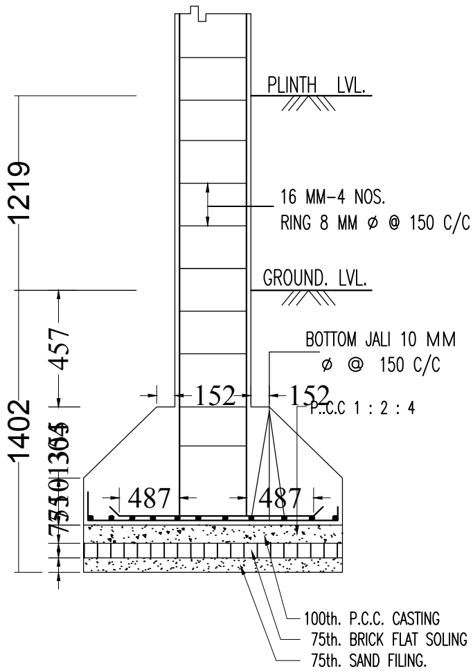
SECTION ON A-A SCALE= 1:50
