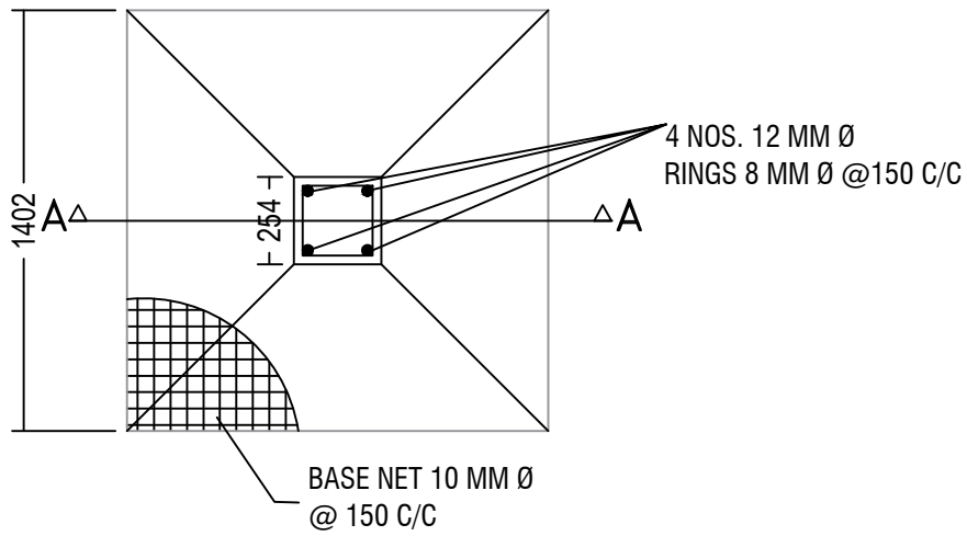
PLAN OF COLUMN FOUNDATION SCALE= 1:50
