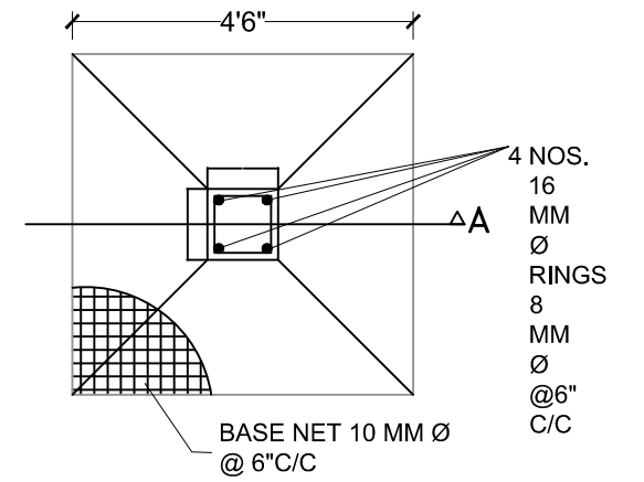
PLAN OF COLUMN FOUNDATION SCALE= 1:50
