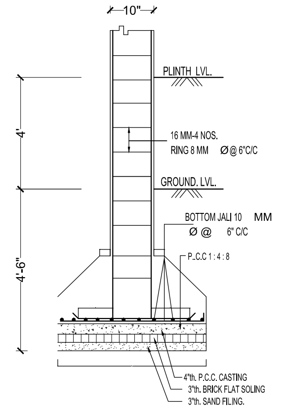
SECTION ON A-A SCALE= 1:50
