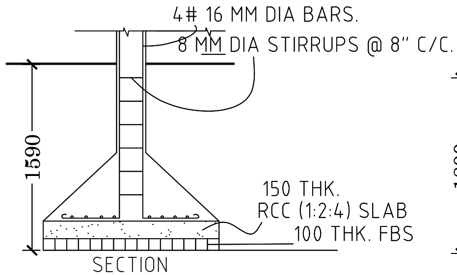
FOUNDATION DETAILS (ISOLATED R.C.C FOOTING)
