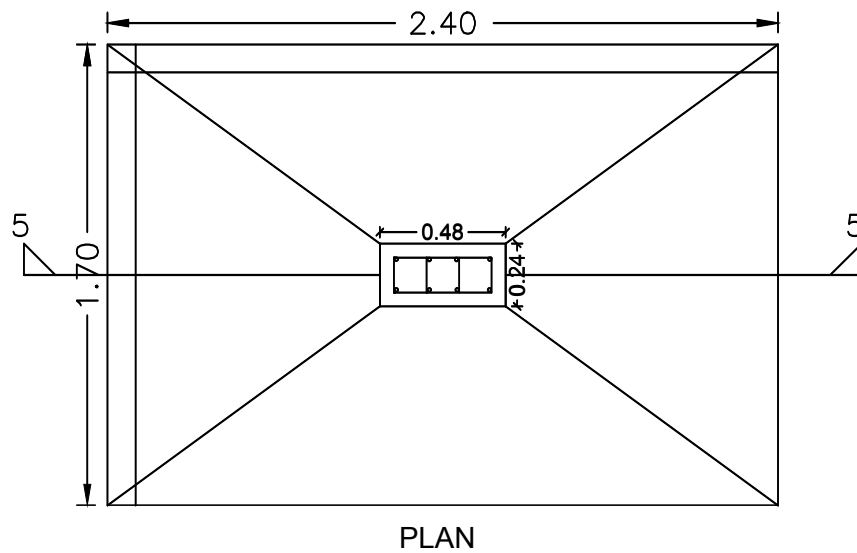
DETAILS OF FOUNDATION SCALE :-1:25
