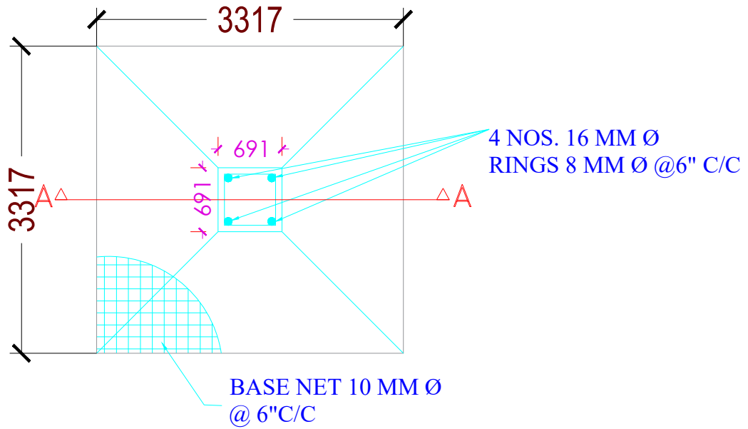
PLAN OF COLUMN FOUNDATION
