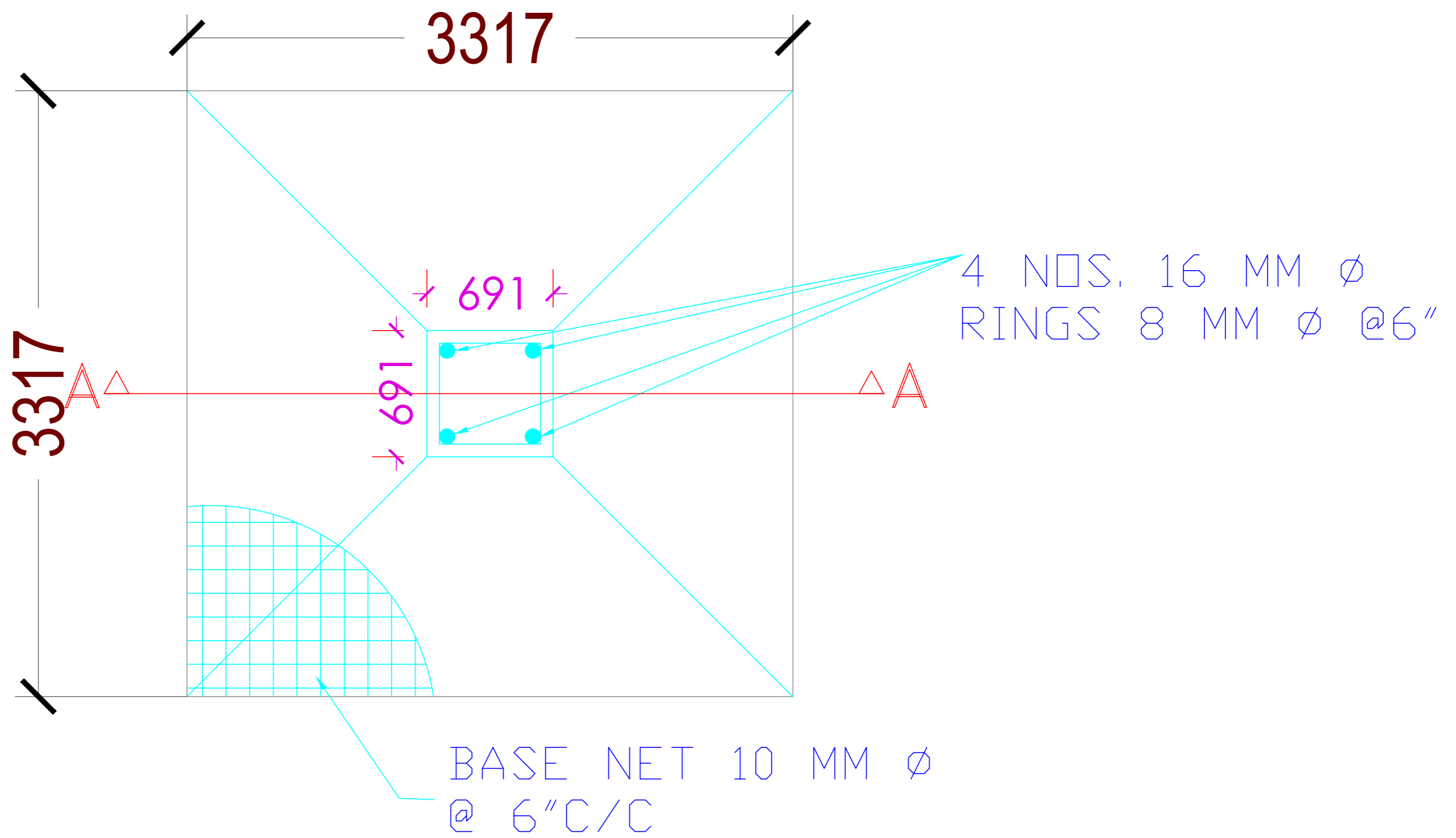
PLAN OF COLUMN FOUNDATION
