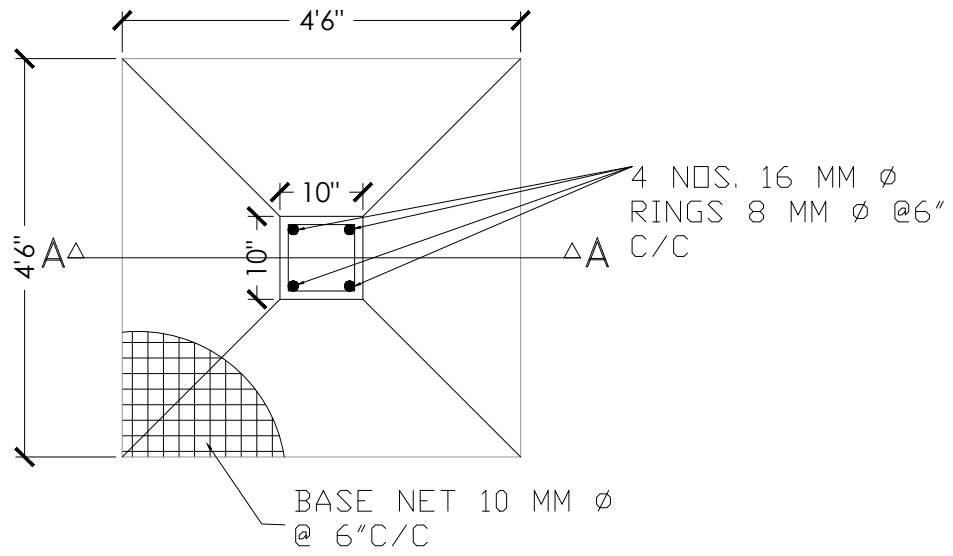
PLAN OF COLUMN FOUNDATION
