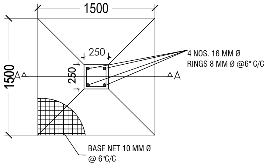
PLAN OF COLUMN FOUNDATION
