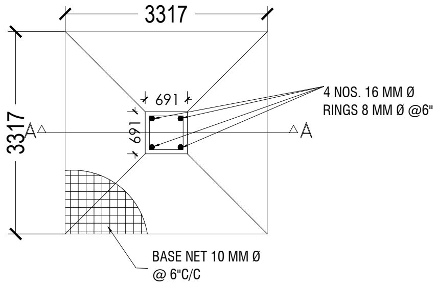
PLAN OF COLUMN FOUNDATION
