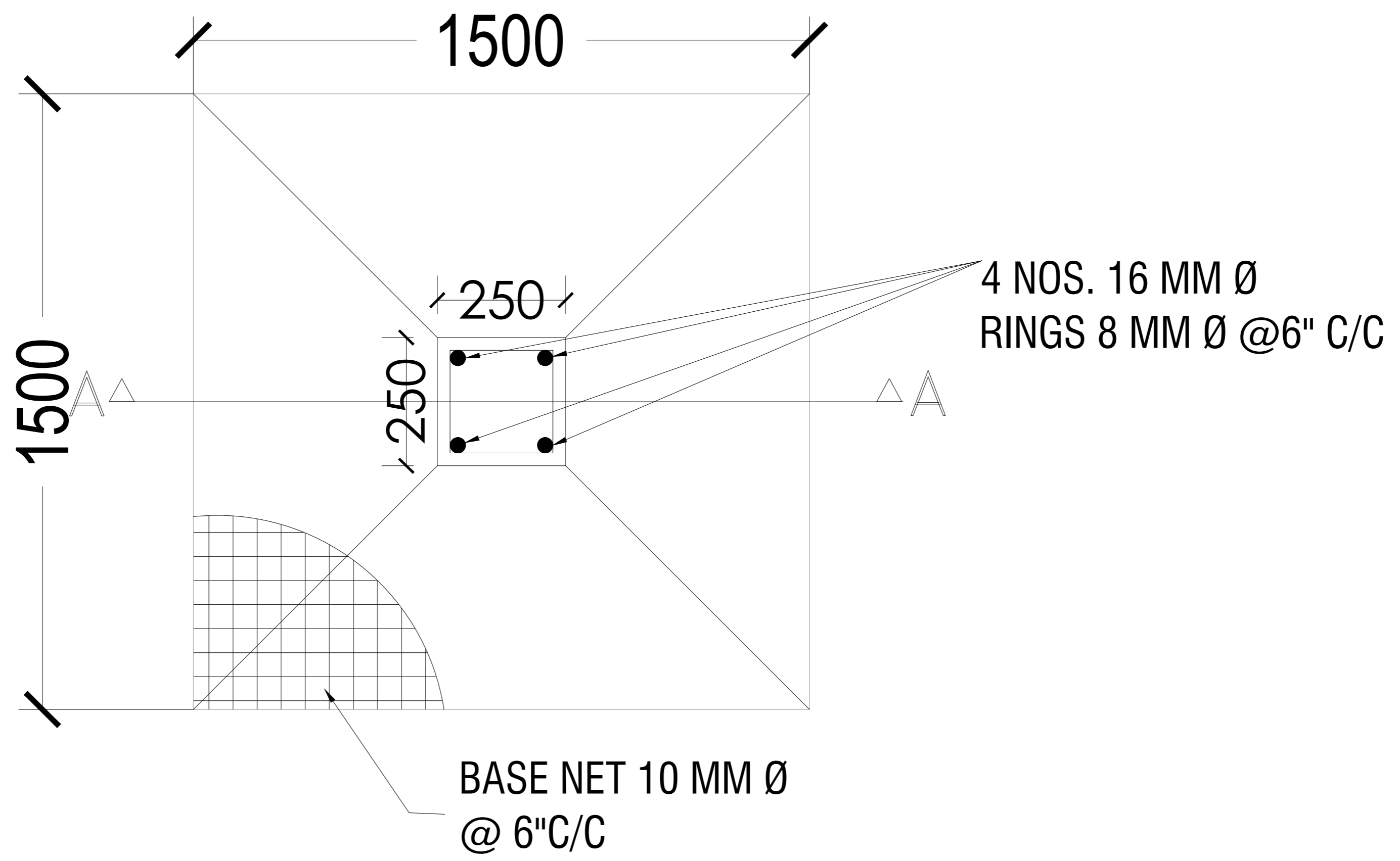
PLAN OF COLUMN FOUNDATION
