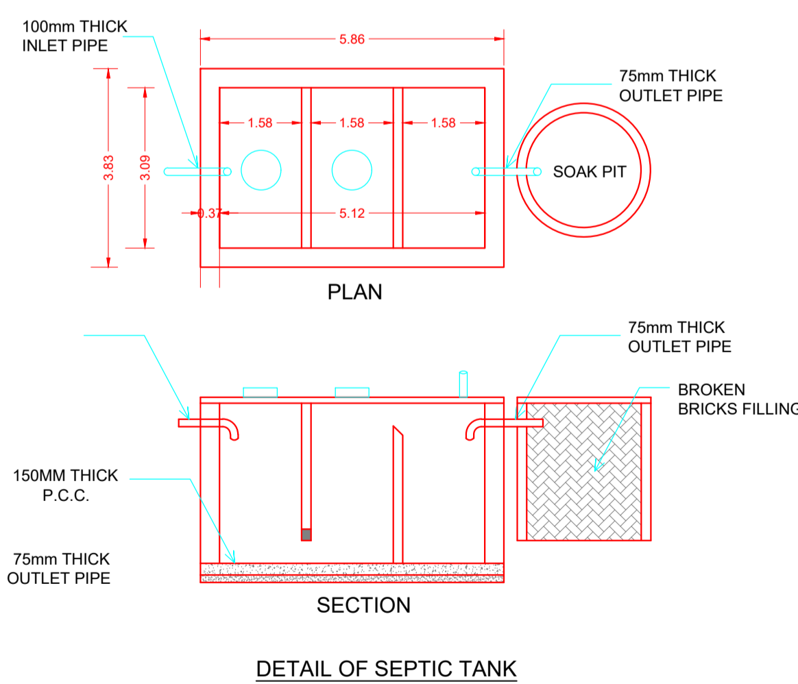
DETAIL OF SEPTIC TANK
