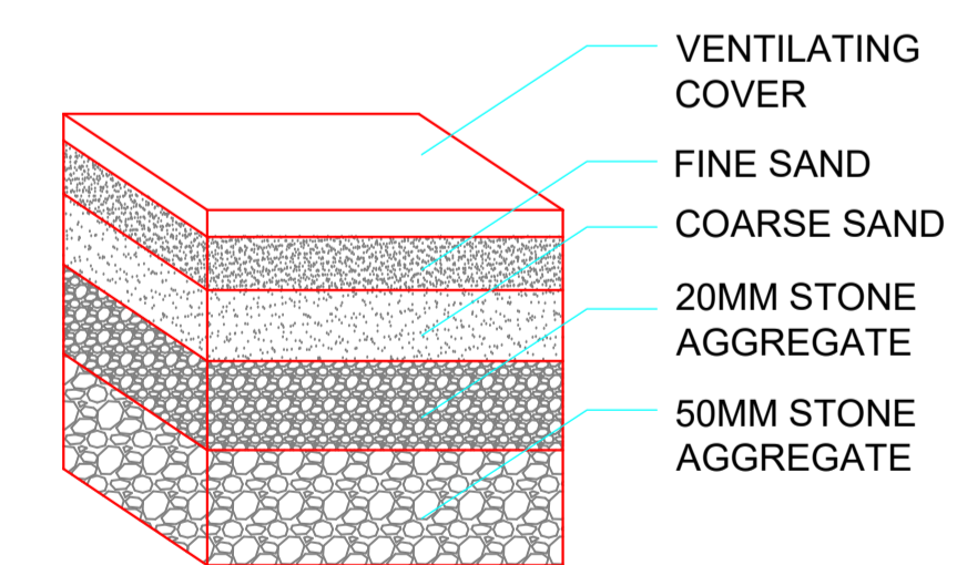
RAIN WATER HARVESTING PIT
