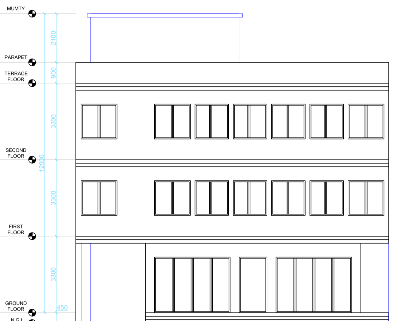
EAST SIDE ELEVATION SCALE - 1:100
