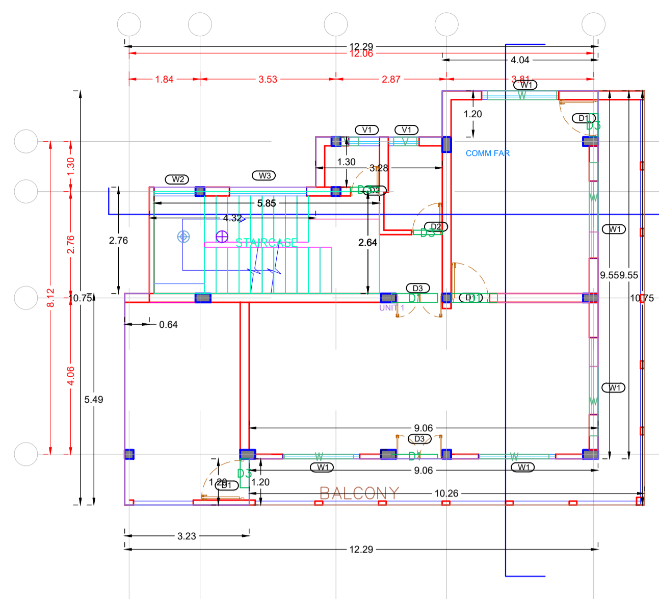
FIRST & SECOND FLOOR PLAN SCALE - 1:100
